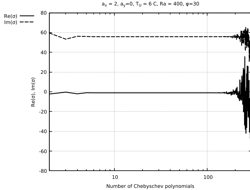
Fig. 1. Sensitivity of eigenvalue calculations on number of polynomials.
