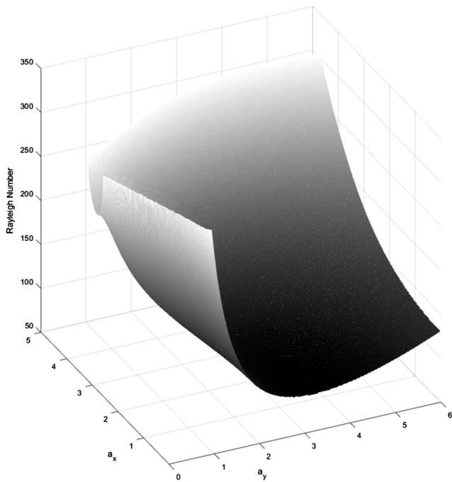
Fig. 4. Critical surface in correspondence of \zeta = 1 ( T_U = 4^\circ\text{C} ) and \phi = 33^\circ .
