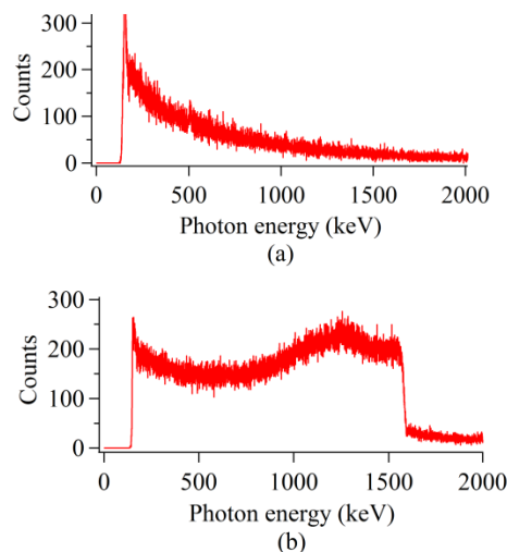
Figure 6: Spectrum at 1.3 GeV for over 120 seconds: (a) radiation background (laser off, e^- beam ~10.7 mA); (b) CBS signal + background (laser on, e^- beam ~9.3 mA).
