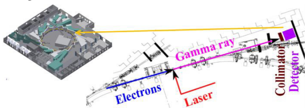
Figure 2: The compact CBS setup for energy measurement at ANKA.
