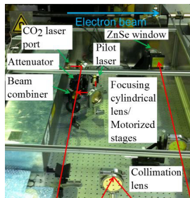
Figure 4: Laser and optical system of the CBS setup.
