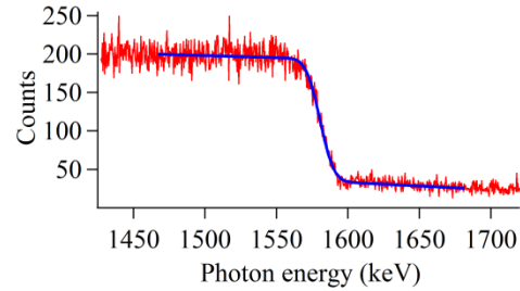
Figure 8: Zoom into Compton edge of Fig. 6 (b) and curve fitting at 1.3 \text{ GeV} , \chi^2/\text{ndf} = 524/555 .
