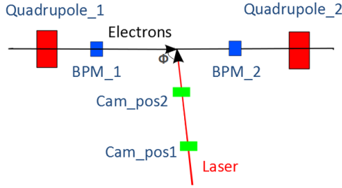
Figure 7: Determination of collision angle.
