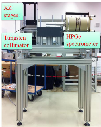
Figure 3: Gamma ray detection system.
