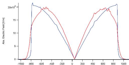
Figure 3: Mode 2 “standing wave” of E-field magnitude for 5 mm IVU gap with tapers (red) and without tapers (blue) along the transverse center line of the IVU. The center zero-crossing indicates clearly a standing wave. At center, the forward and backward waves cancel. At the |E| peaks they add.
