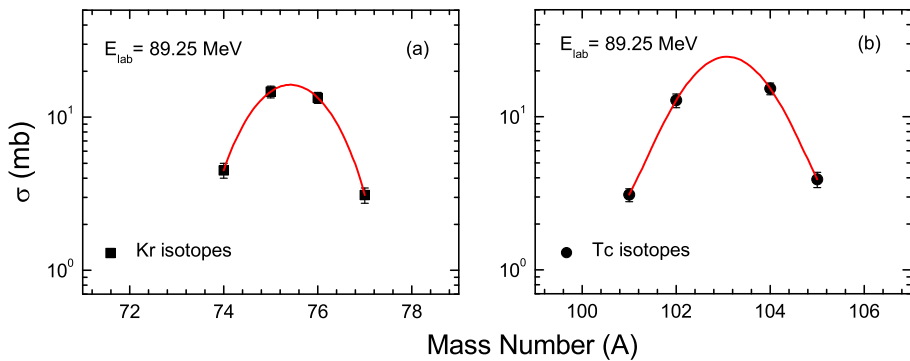
Fig. 1. (a) Isotopic yield distribution, and (b) fractional independent yield distribution of Kr isotopes at E_{\text{lab}} = 89.25 MeV. The solid lines are the fitted Gaussian distribution.
