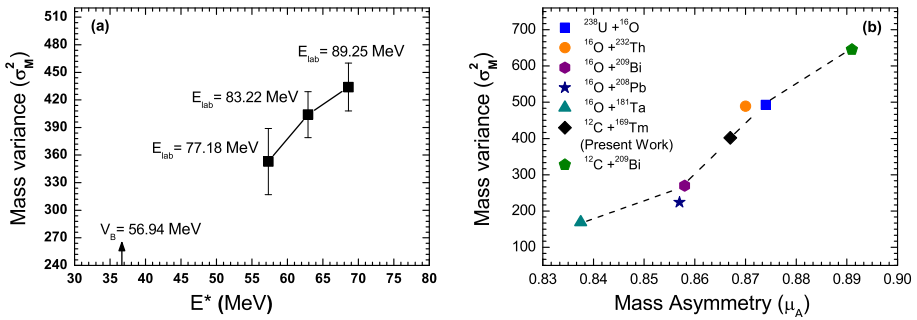
Fig. 2. (a) Variation of mass distribution with excitation energy ( E^* ) for deformed thulium target. The arrow points to E^* corresponding to Coulomb barrier. (b) Mass variance ( \sigma_M^2 ) as a function of mass asymmetry for different projectile–target system. The solid and dashed lines are drawn to guide the eyes.
