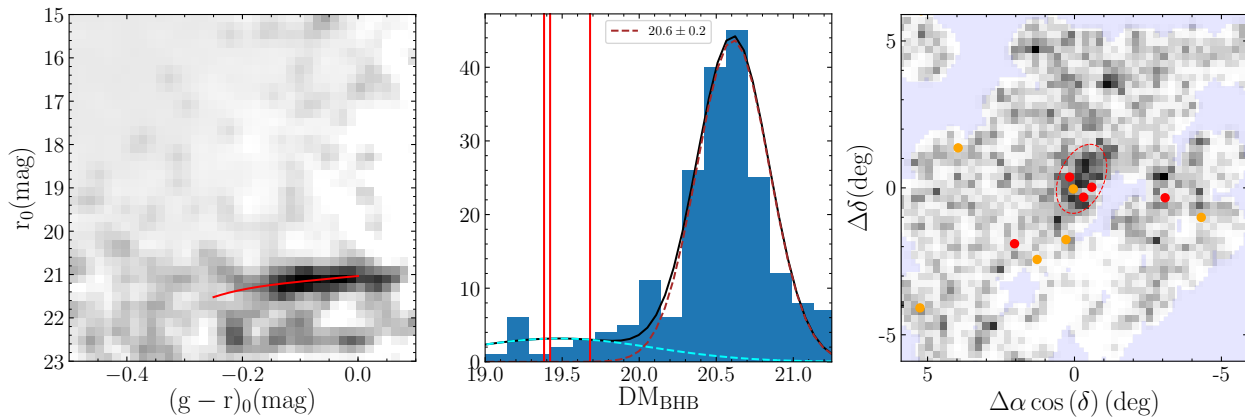
Figure 3. BHBs and RR Lyrae stars in Antlia 2. Left: DECam Hess difference (difference of CMD densities) of the stars within the Ant 2's half-light radius and the foreground, zoomed in on the BHB region. The red line shows the BHB ridge-line as given in Deason et al. (2011) at the best fit distance modulus. Middle: Distribution of the distance moduli of the selected BHB candidates, along with the best-fit two-Gaussian plus a flat background model. The vertical lines mark the distance moduli of the four RRL stars within the half-light radius of the satellite. Right: On-sky density distribution of the BHB candidates. RRL stars with heliocentric distances larger than 70 kpc are shown in red, stars with distances between 55 and 70 kpc are shown in orange.
