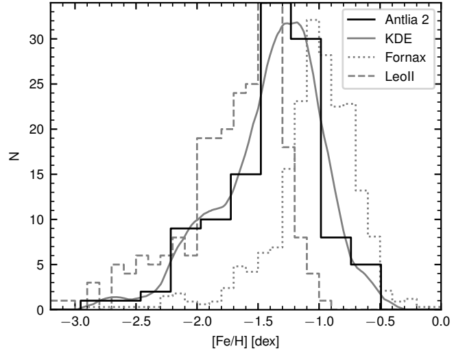
Figure 10. Distribution of spectroscopic metallicities of Ant 2's stars with 274 < \text{HRV} < 303 km/s and metallicity error less than 0.5 dex. The black line is the [\text{Fe}/\text{H}] histogram with a bin size of 0.2 dex, while the grey curve shows the kernel density estimation using the Epanechnikov kernel. The mean metallicity is \langle [\text{Fe}/\text{H}] \rangle = -1.36 , with a significant scatter toward low metallicities. Metallicity distributions of stars in Fornax and Leo II are also shown for comparison.
