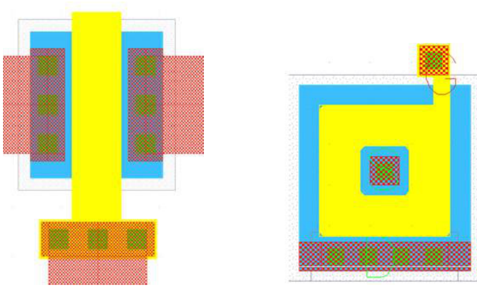
Figure 1. Shown on the left is the layout of a standard CMOS transistor while on the right is the layout of an enclosed (or circular) transistor.
