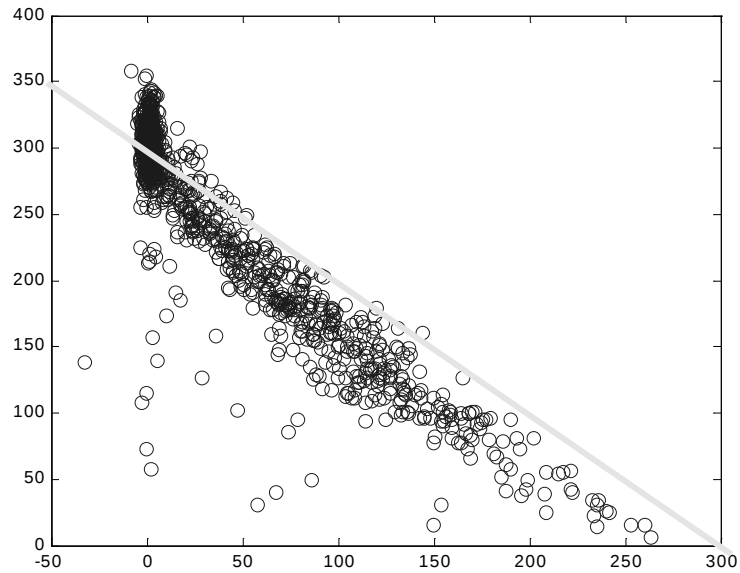
Figure 6: Data on the ECAL and HCAL response to a beam of 300 GeV pions. The line indicates the response expected for a linear calorimeter. Clearly, there is a mismatch in e/h between the 2 compartments. This mismatch projected onto the total energy response induces additional error.
