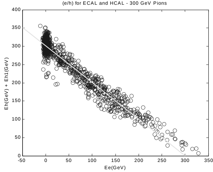
Figure 8: Data for 300 GeV pions using the determination of e/h for both the ECAL and HCAL compartments and correcting the response for the electron to pion ratio in both compartments event by event.
