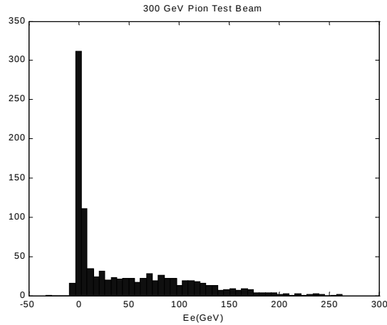
Figure 2: Energy in the ECAL compartment for 300 GeV pions incident on the ECAL + HCAL.
