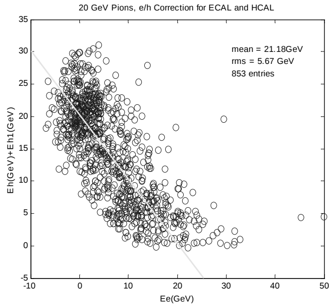
Figure 9: Data for 20 GeV pions using the determination of e/h for both the ECAL and HCAL compartments and correcting the response for the electron to pion ratio in both compartments event by event. The line indicates the response of a linear overall device.
