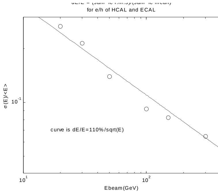
Figure 12: Sample r.m.s of the energy distribution divided by the mean for pions detected in ECAL + HCAL after correction for the e/h of the two compartments. The line represents a stochastic coefficient of 110%.
