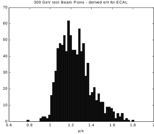
Figure 7: Derived value of the electron to pion ratio for the ECAL compartment for 300 GeV pion events which deposit > 100 GeV in the ECAL compartment.
