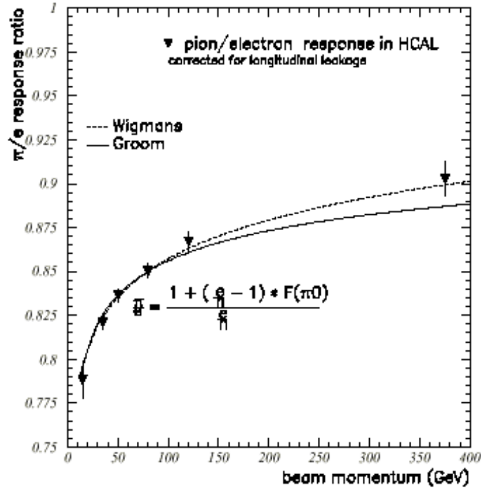
Figure 4: HCAL pion energy response (mean) as a function of test beam energy and the fit to that response using e/h = 1.39 . Note that the data shown here is normalized such that the pion to electron response at 300 GeV is \sim 0.90 and not = 1 as it was in Figure 1.
