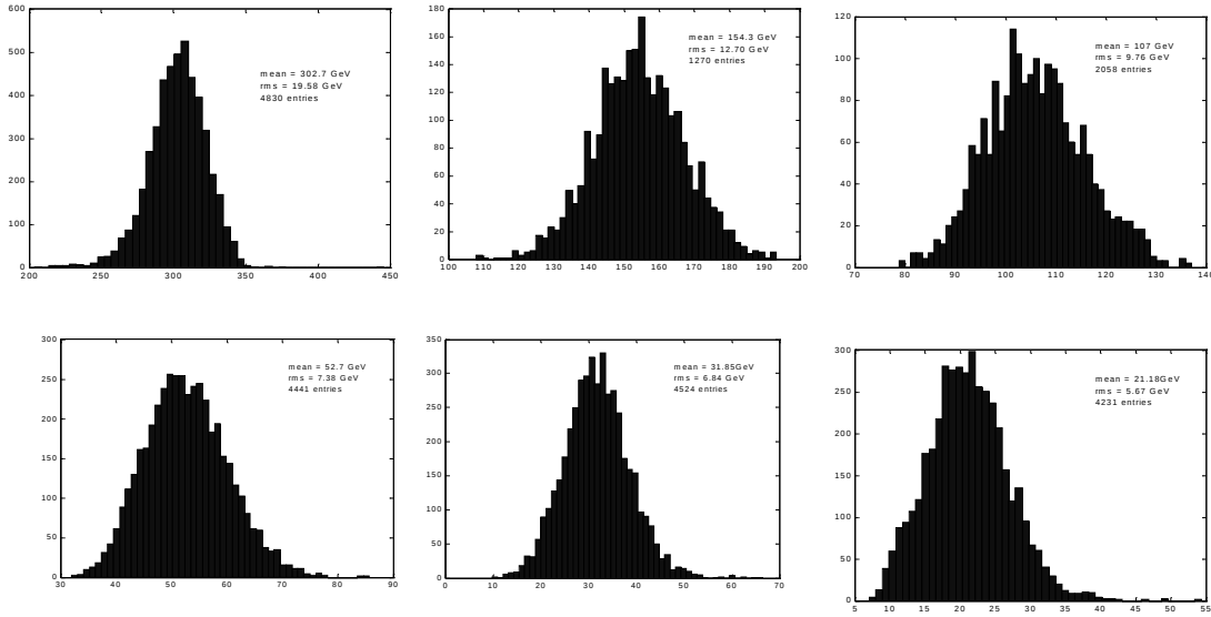
Figure 10: Distributions of the sum of the corrected energies for ECAL plus HCAL for incident pion beams of 20, 30, 50, 100, 150, and 300 GeV.
