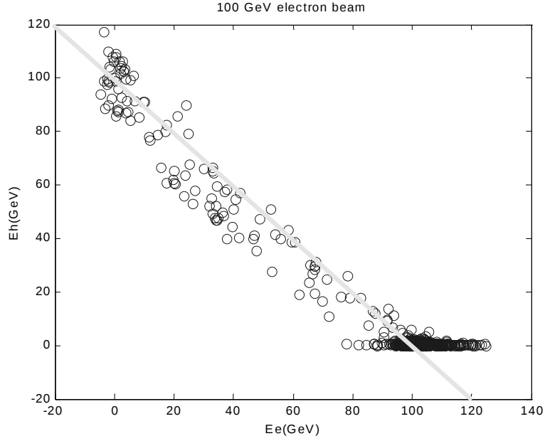
Figure 5: Data on the ECAL and HCAL response to a beam of 100 GeV electrons. The line indicates the response expected for a linear calorimeter. Aside from the pion contamination in the beam, the full beam energy is deposited in ECAL.
