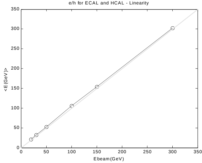
Figure 11: Mean of the energy detected in ECAL + HCAL after correction for the e/h of the two compartments. The line is a linear detector response.
