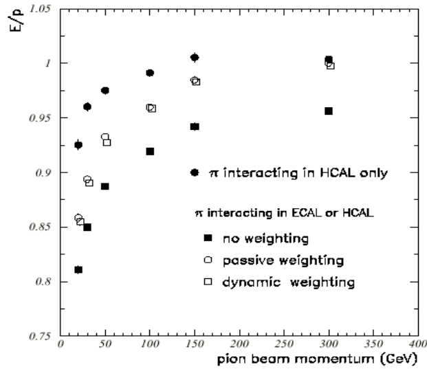
Figure 1: The response of the HCAL to pions of a given momentum in a test beam. The quantity plotted is the energy response divided by the beam energy ( equal to the electron response assuming a linear calorimeter for electromagnetic energy deposits).
