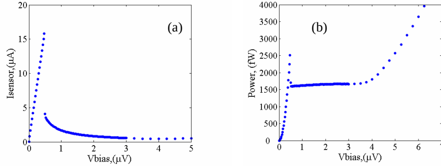
Fig. 4. Current (a) and power (b) as a function of voltage bias, respectively. Below 3 \mu\text{V} the sensor is self-biased, and the power is approximately constant as a function of voltage. Device base temperature is \sim 72 mK.
