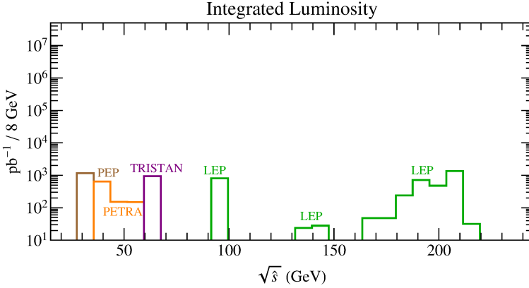
Fig. 9. Gaps in e^+e^- integrated luminosity coverage left by PEP, PETRA, TRISTAN and LEP at center-of-mass energies above B factories.
