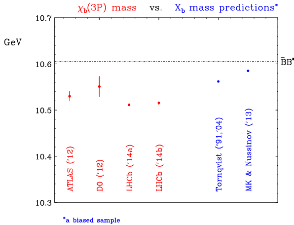
Fig. 5. Comparison of measured values of \chi_{b1}(3P) mass with predicted values of X_b mass.
