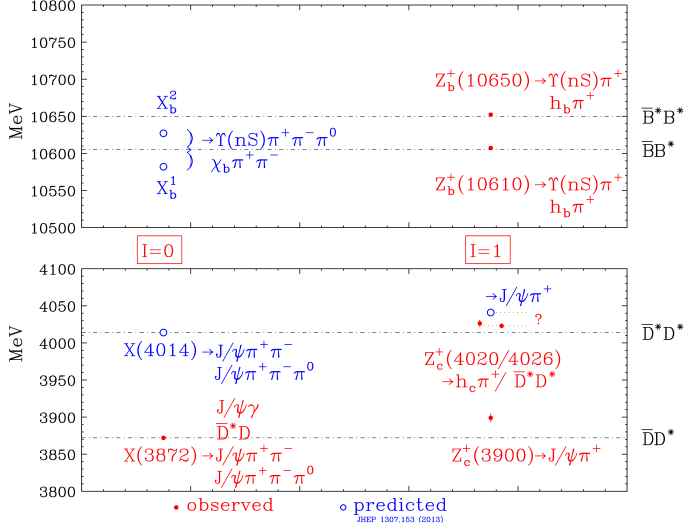
Fig. 4. Decay channels of doubly-heavy exotic quarkonia. The legend is as in figure 3.
