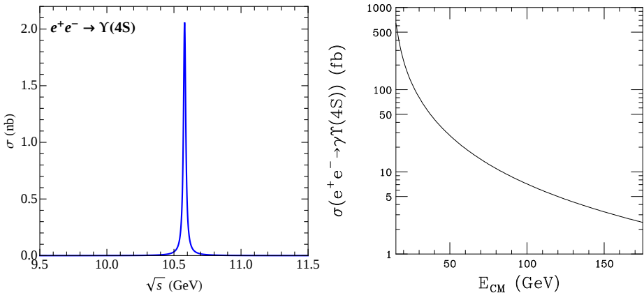
Fig. 11. Cross section for e^+e^- \rightarrow \Upsilon(4S) (left) and including the emission of a photon at an e^+e^- collider with CM energy E_{\text{CM}} (right).
