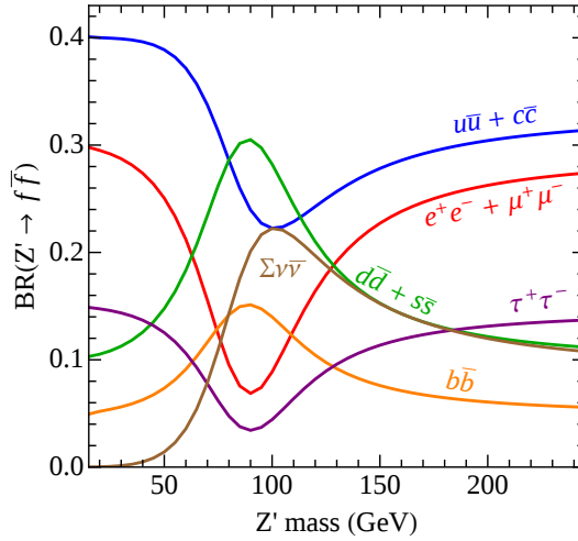
Fig. 16. Dark photon branching ratios. These are computed using \epsilon = 5 \times 10^{-3} although for \epsilon \ll 1 the branching ratios are independent of \epsilon .
