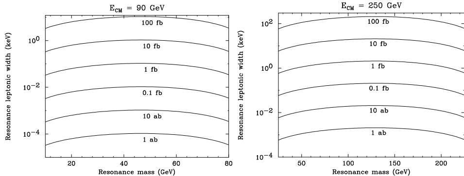
Fig. 12. Contours of equal cross section for radiative return production of a resonance with leptonic width \Gamma_{ee} (assuming 100% branching fraction to a final state f ). Left: E_{\text{CM}} = 90 GeV; right: E_{\text{CM}} = 250 GeV.
