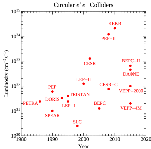
Fig. 10. Maximum instantaneous luminosities of circular e^+e^- colliders versus time. Adapted from Fig. 1 of Ref. [62].
