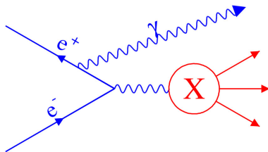
Fig. 8. Schematic depiction of the radiative return process in an e^+e^- collider. Before the collision, one of the leptons emits a hard photon, thereby significantly reducing the center-of-mass energy of available for e^+e^- annihilation into the final state X .
