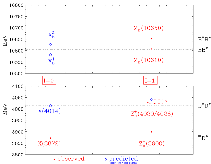
Fig. 3. Masses of the doubly-heavy exotic quarkonia vs. two-meson thresholds. The states observed so far are shown in gray/red, the predicted states are shown in black/blue. I = 0 resonances are shown on the left and isovectors are shown on the right. Note the proximity of all the states to the corresponding two-meson thresholds.
