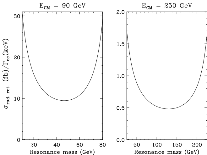
Fig. 13. \sigma(e^+e^- \rightarrow \gamma R \rightarrow \gamma f)/\Gamma_{ee}\mathcal{B}_f as a function of resonance mass for E_{\text{CM}} = 90 (left) and 250 (right) GeV.
