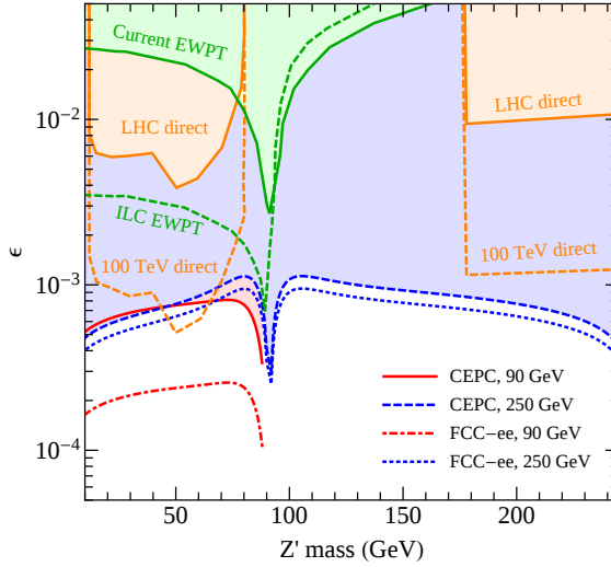
Fig. 17. Dark photon limits at 95% C.L. on the hypercharge mixing \epsilon as a function of dark photon mass. The \sqrt{s} = 90 GeV and 250 GeV lines show our projections with future e^+e^- colliders with integrated luminosities specified in Table VI. Electroweak precision constraints (EWPT) and direct searches are taken from [65]. The 100 TeV projection assumes an integrated luminosity of 3000 \text{ fb}^{-1} .
