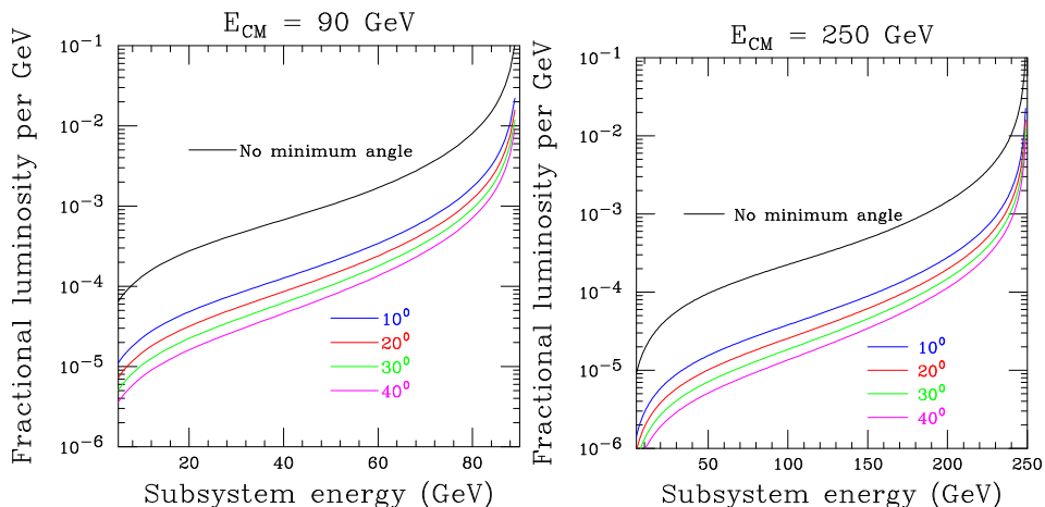
Fig. 14. Fractional luminosity L_f as a function of subsystem energy \hat{E}_{\text{CM}} for E_{\text{CM}} = 90 (left) and 250 (right) GeV. Top curves: No minimum angle; infrared cutoff provided by \ln(E/m_e) [Eq. (13)]. Lower curves, top to bottom: \theta_0 = 10, 20, 30, 40^\circ .
