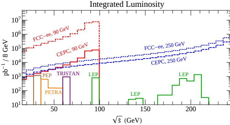
Fig. 15. Integrated luminosity from past low energy e^+e^- colliders at their nominal center-of-mass energies compared to the effective luminosity through radiative return from future e^+e^- colliders at \sqrt{s} = 90 or 250 GeV (no minimum angle; see Fig. 14 for effects of minimum angles). The FCC-ee curves assume an integrated luminosity of 50 \text{ab}^{-1} at 90 GeV and 10 \text{ab}^{-1} at 250 GeV. The CEPC curves assume an integrated luminosity of 0.5 \text{ab}^{-1} at 90 GeV and 5 \text{ab}^{-1} at 250 GeV. Integrated luminosities of PEP-II and Belle (Table VII) exceed those achievable by radiative return at FCC-ee or CEPC running at 90 or 250 GeV.
