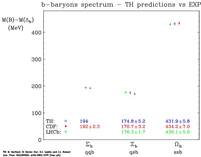
Fig. 7. Masses of b baryons — comparison of theoretical predictions [33, 34] with experiment.
