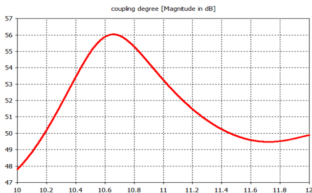
Figure 10: Coupling degree of circular-rectangle waveguide directional coupler by CST.
