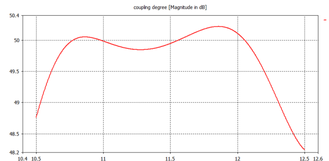
Figure 6: Coupling degree of H-plane directional coupler by CST.
