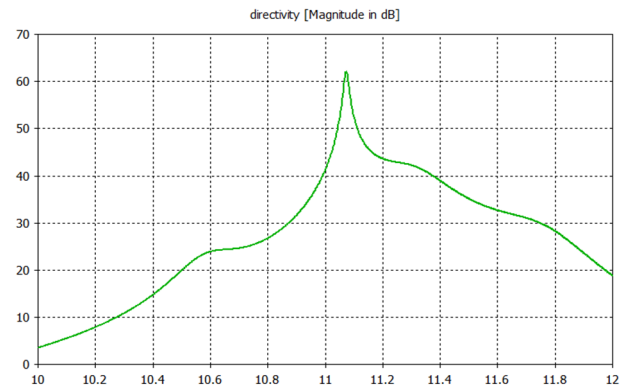
Figure 11: Directivity of circular-rectangle waveguide directional coupler by CST.
