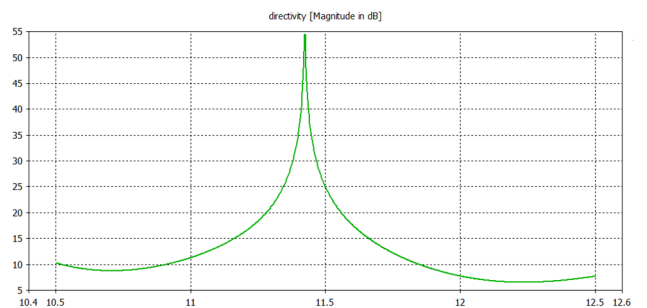
Figure 7: Directivity of H-plane directional coupler in CST.
