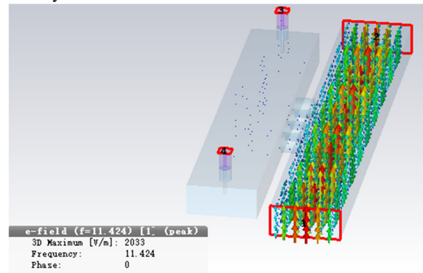
Figure 5: Electric field of H-plane directional coupler by CST.
