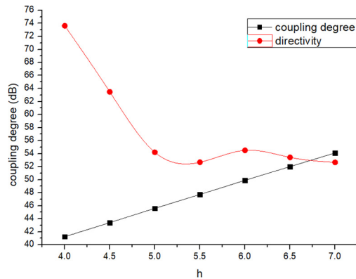
Figure 3: Curves of coupling degree and directivity with respect to the height of the hole.
