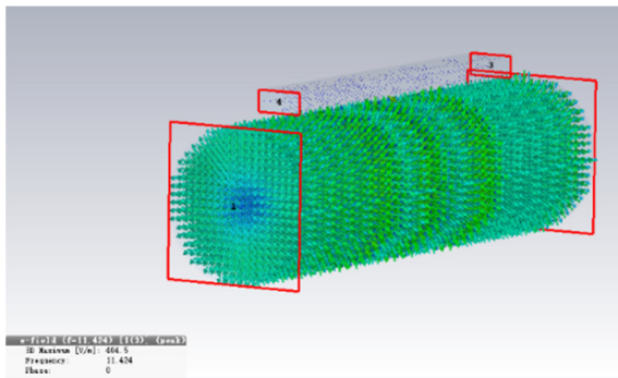
Figure 9: Electric field of circular-rectangle waveguide directional coupler by CST.
