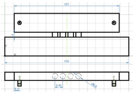
Figure 4: Main dimensions of H-plane directional coupler (units: mm).
