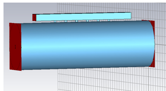
Figure 8: Circular-rectangle waveguide directional coupler in CST.
