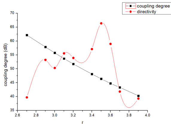
Figure 2: Curves of coupling degree and directivity with respect to the radius of the hole.
