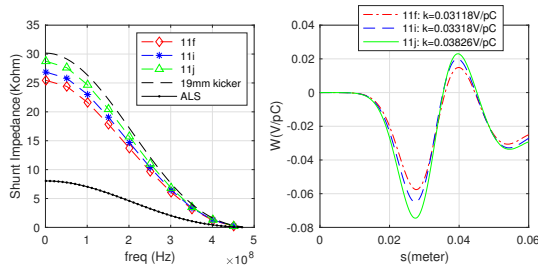
Figure 4: Shunt impedance (left) and loss factor (right).
