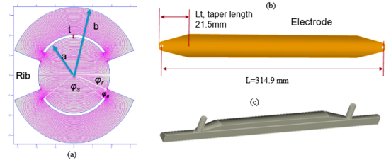
Figure 3: Numerical models for 2D and 3D simulations: (a), Poisson model; (b), the electrode in the 3D model; (c), the 3D model.
