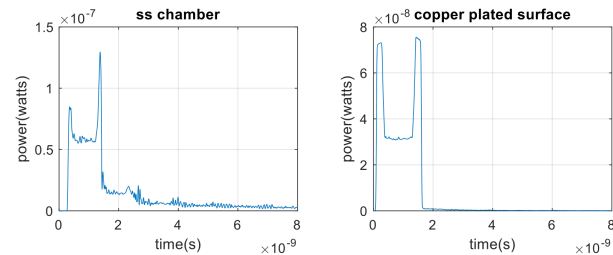
Figure 6: Surface power dissipation for kicker design 11j.
