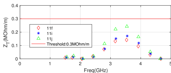
Figure 5: Trapped horizontal modes in the vertical kicker.
