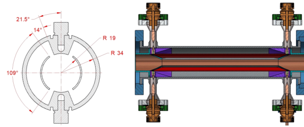
Figure 1: Overview of the TMBF kicker design: the cross section of the nominal section (left) and the cut away view of the whole structure (right).
