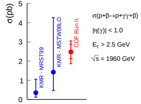
FIG. 4. Comparison of the measured cross section for the exclusive \gamma\gamma production in p\bar{p} collisions at \sqrt{s} = 1.96 TeV with theoretical predictions [9].
