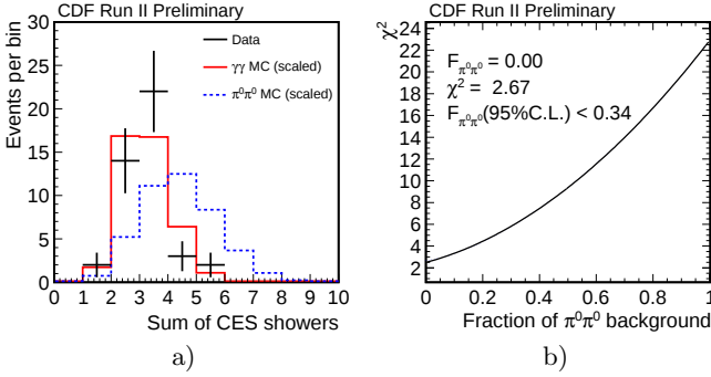
FIG. 3. Estimate of \pi^0\pi^0 background fraction in the candidate sample. Distribution of reconstructed CES showers per event for data compared to \gamma\gamma and \pi^0\pi^0 Monte Carlo (a). Background fraction estimate using Pearson's \chi^2 test to fit the composition hypothesis to the data distribution (b).
