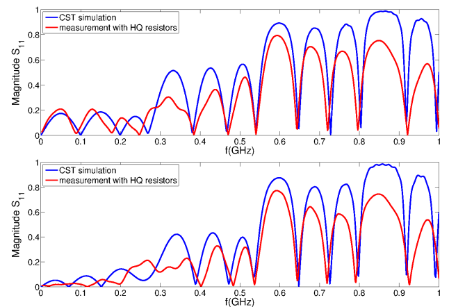
Figure 1: S_{11} parameter measured when driving the electrodes in the odd (top) or even (bottom) mode configuration, when output is terminated with the HQ terminating resistors, compared with CST simulations.
