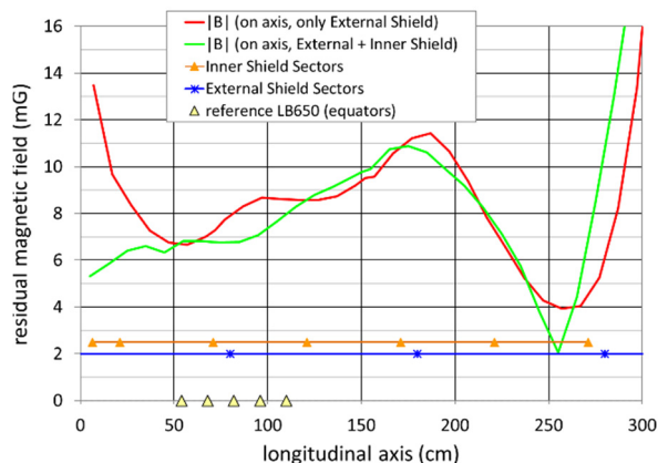
Figure 4: Magnetic field vector amplitude as measured along the LASA cryostat vertical axis in different shielding configurations.
