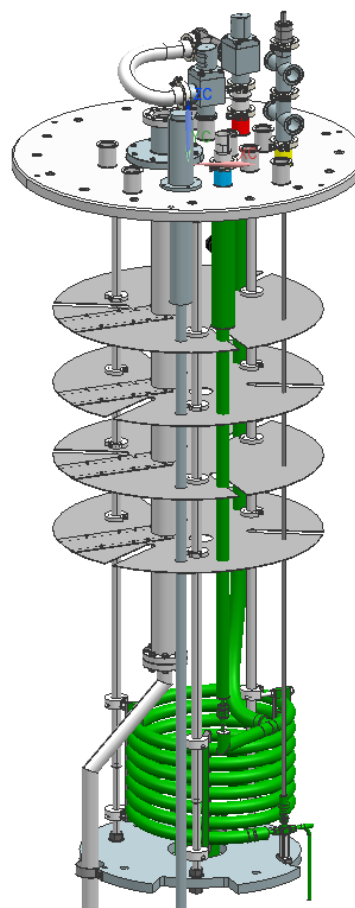
Figure 5: CAD view of Heat-Exchanger, J-T valve and related process lines on the LASA LB650 vertical insert.
