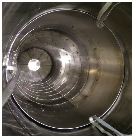
Figure 3: Cryoperm ® magnetic shielding in place inside the vertical testing cryostat. A second, external shield at room temperature is placed (not visible here) around the cryostat.
