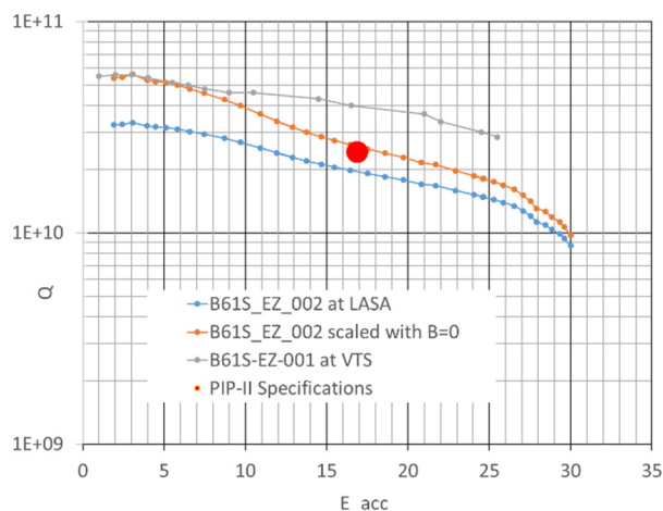
Figure 1: Q -vs- E_{\text{acc}} results for the two INFN LB650 single cell cavities, compared to PIP-II specifications.
