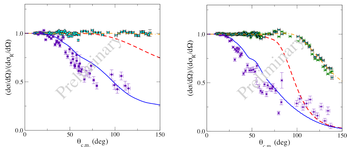
Figure 5. (color online) Differential elastic cross section of ^9\text{Li} and ^{11}\text{Li} on ^{208}\text{Pb} for CM energies of 23.0 MeV on the left, and 28.2 MeV on the right. The results obtained for ^9\text{Li} on ^{208}\text{Pb} are given for both targets. For details on the calculations see text.
