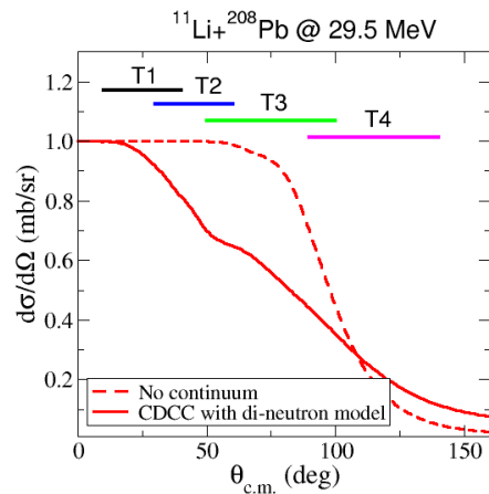
Figure 2. Expected CDCC differential elastic cross section relative to Rutherford of ^{11}\text{Li} on ^{208}\text{Pb} at 29.5 MeV. The coverage of each telescope is indicated in the upper part.
