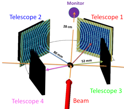
Figure 1. (color online) Schematic view of the experimental setup. The angular coverage of each telescope from T1 to T4 is: 10^\circ - 40^\circ , 30^\circ - 60^\circ , 50^\circ - 100^\circ and 90^\circ - 140^\circ , respectively.
