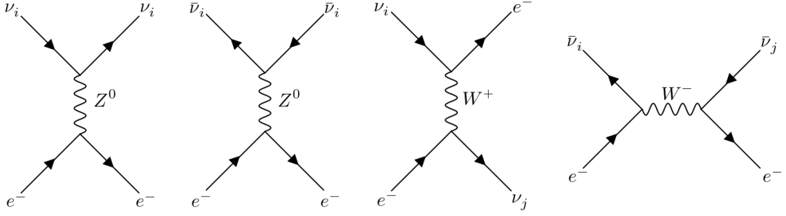
Figure 14. Tree level diagrams contributing to the scattering of neutrino mass eigenstate i on electrons.
