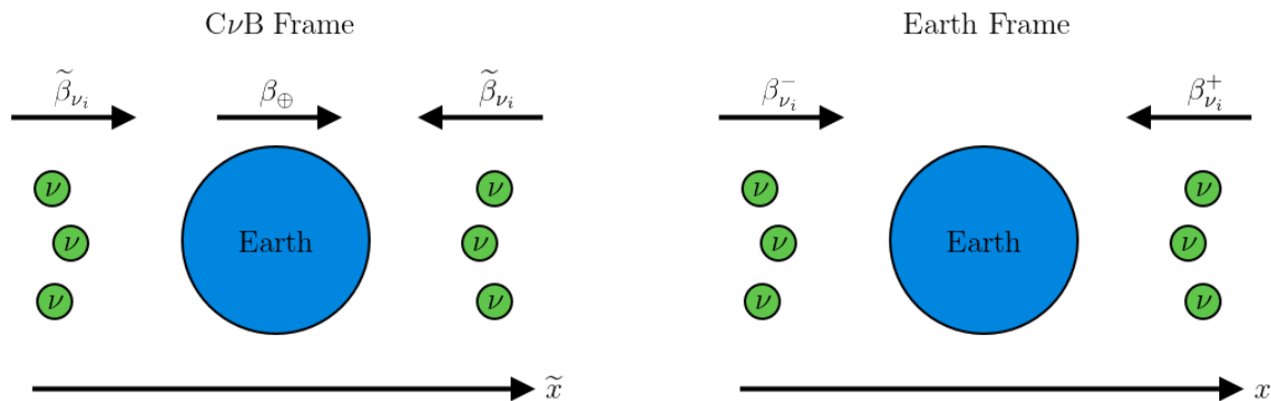
Figure 2. 1-dimensional setup used to estimate the average momentum transfer by each scattering event, \Delta p_{\nu_i} , in [18]. Left: the Earth moves at velocity \beta_{\oplus} relative to the C\nu B frame, where neutrinos have mean velocity \tilde{\beta}_{\nu_i} . Right: in the Earth’s reference frame, neutrinos move with velocity \beta_{\nu_i}^+ or \beta_{\nu_i}^- , generating a lab frame asymmetry in the C\nu B .
