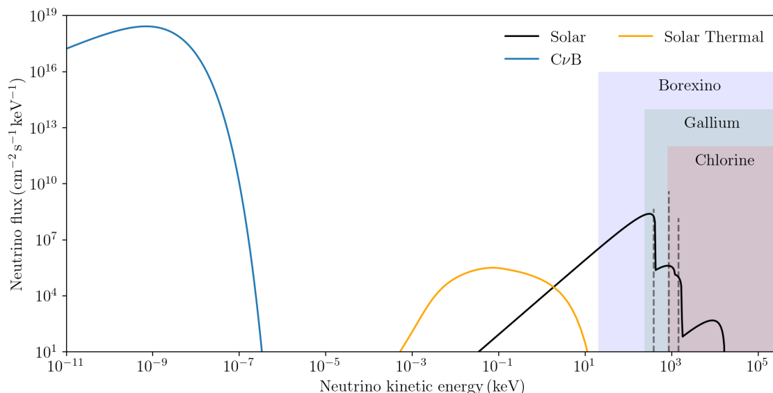
Figure 1. Predicted electron neutrino flux from the C\nu B (blue), alongside those from nuclear (black) and thermal (orange) processes in the sun, assuming degenerate neutrino mass m_\nu = 0.1 eV. We also show the energy thresholds for neutrino detection at gallium and chlorine radiochemical experiments, alongside the threshold at Borexino [4]. For a comprehensive review of neutrino fluxes at all energies, see [5].
