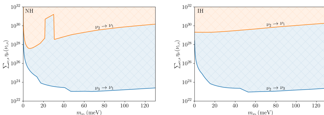
Figure 7. Bounds that could be set on the decaying relic neutrino overdensity by LIM experiments as a function of the lightest neutrino mass. For all values of the mass, we use the best experimental sensitivity of COMAP [127], CCAT-prime [128] and AtLAST [129] as given in [126], and assume the theoretical decay width (5.89), with effective electromagnetic moment (5.91). Left: in the normal mass hierarchy. Right: in the inverted mass hierarchy.
