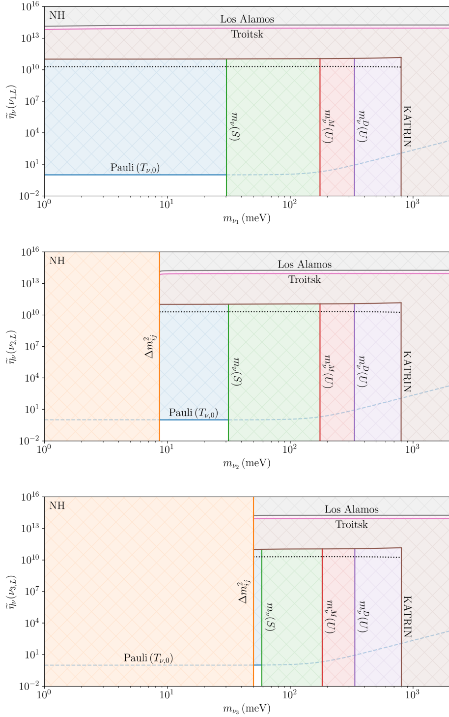
Figure 3. Present day constraints on the CνB frame relic neutrino overdensity in the normal mass hierarchy, assuming the standard scenario and \beta_{\oplus} = \beta_{\oplus}^{\text{CMB}} . The KATRIN, Troitsk and Los Alamos overdensity bounds shown assume Dirac neutrinos, and are stronger by a factor of two under the Majorana neutrino hypothesis. See the text for a full description of the figure.
