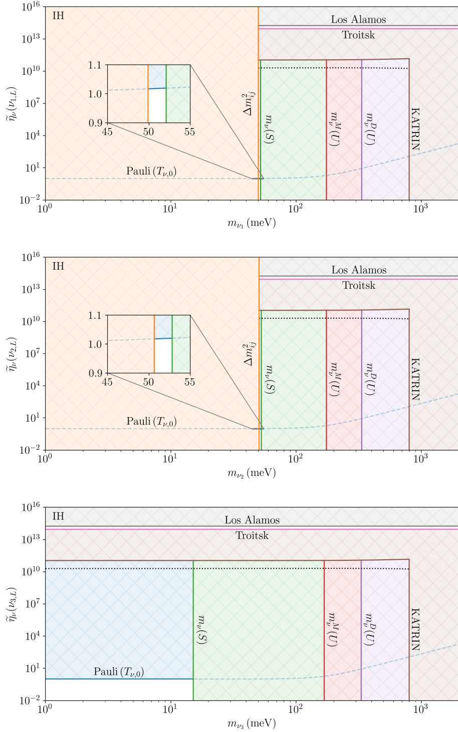
Figure 4. Present day constraints on the C\nu B frame relic neutrino overdensity in the inverted mass hierarchy, assuming the standard scenario and \beta_\oplus = \beta_\oplus^{\text{CMB}} . The KATRIN, Troitsk and Los Alamos overdensity bounds shown assume Dirac neutrinos, and are stronger by a factor of two under the Majorana neutrino hypothesis. See the text for a full description of the figure.
