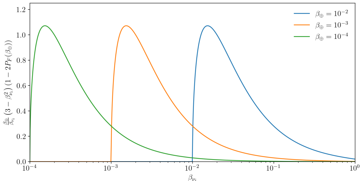
Figure 6. Helicity term appearing in the Stodolsky effect energy shifts for a range of reference frame velocities, \beta_{\oplus} . As the neutrino velocity, \beta_{\nu_i} , approaches the Earth’s velocity, the term vanishes identically.
