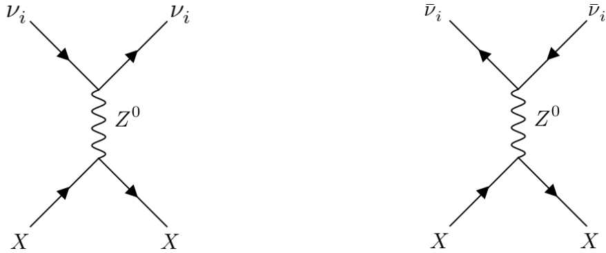
Figure 13. Tree level diagrams contributing to the scattering of (anti)neutrino mass eigenstate i on nucleus X . The Majorana neutrino amplitude is found by taking the difference between these two diagrams.
