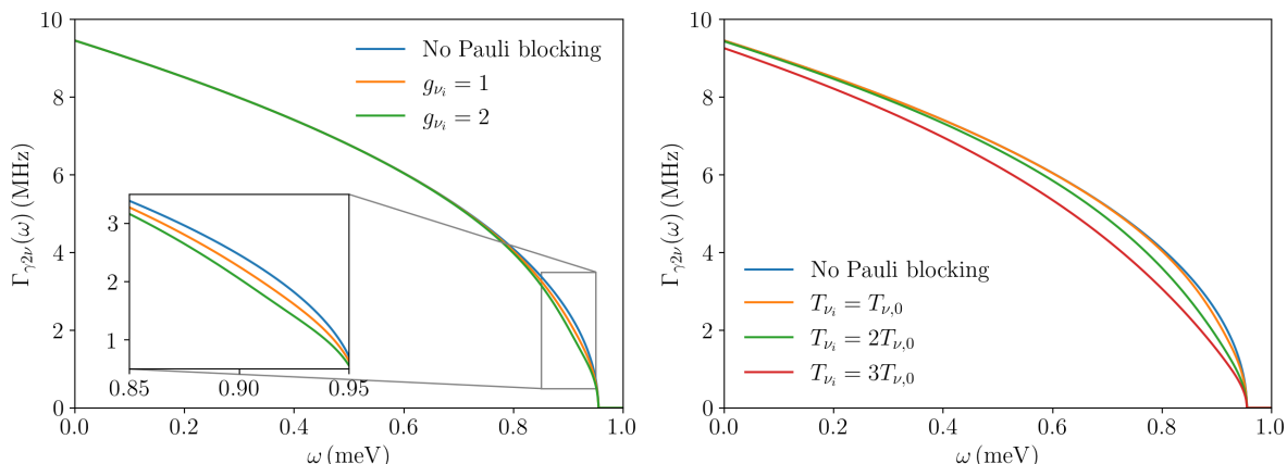
Figure 8. RENP photon energy spectrum in the presence of the C\nu B for the toy ‘Cs-like’ system described in the text, where n_T = 10^{21} \text{ cm}^{-3} , V = 100 \text{ cm}^3 and the lightest neutrino mass m_{\nu_i} = 5 \text{ meV} . Left: varying the neutrino degeneracy parameter, g_{\nu_i} , at constant temperature T_{\nu_i} = T_{\nu,0} . Right: varying the neutrino temperature, T_{\nu_i} in multiples of the standard temperature, T_{\nu,0} = 0.168 \text{ meV} , with g_{\nu_i} = 1 . In both plots, we assume Dirac neutrinos in the normal mass hierarchy.
