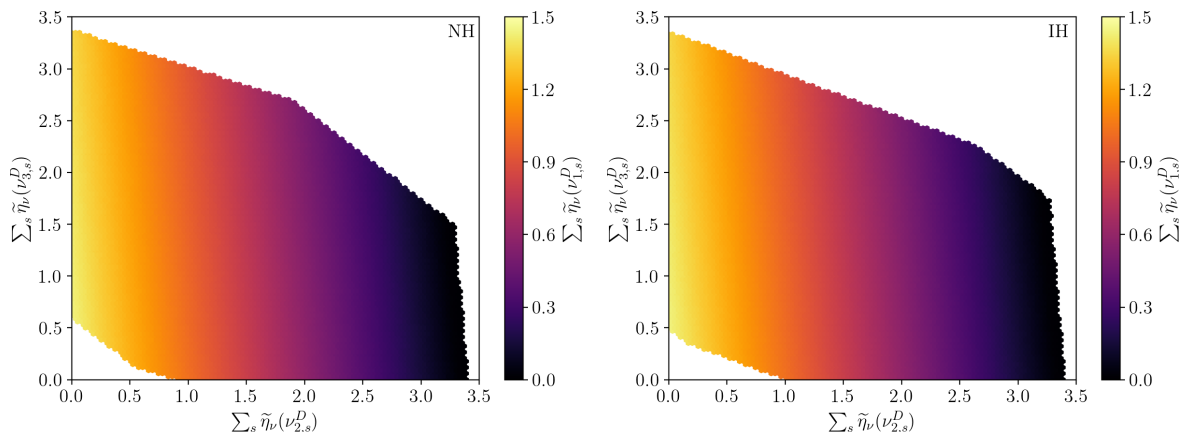
Figure 5. Cosmological constraints on the relic neutrino overdensity due to a degeneracy parameter \xi_{\nu_i} in the \sum_s \tilde{\eta}_\nu(\nu_{2,s}) - \sum_s \tilde{\eta}_\nu(\nu_{3,s}) plane, where the colour shows the mean allowed magnitude of \sum_s \tilde{\eta}_\nu(\nu_{1,s}) . Any point in the white regions is excluded. Left: in the normal mass hierarchy. Right: in the inverted mass hierarchy.
