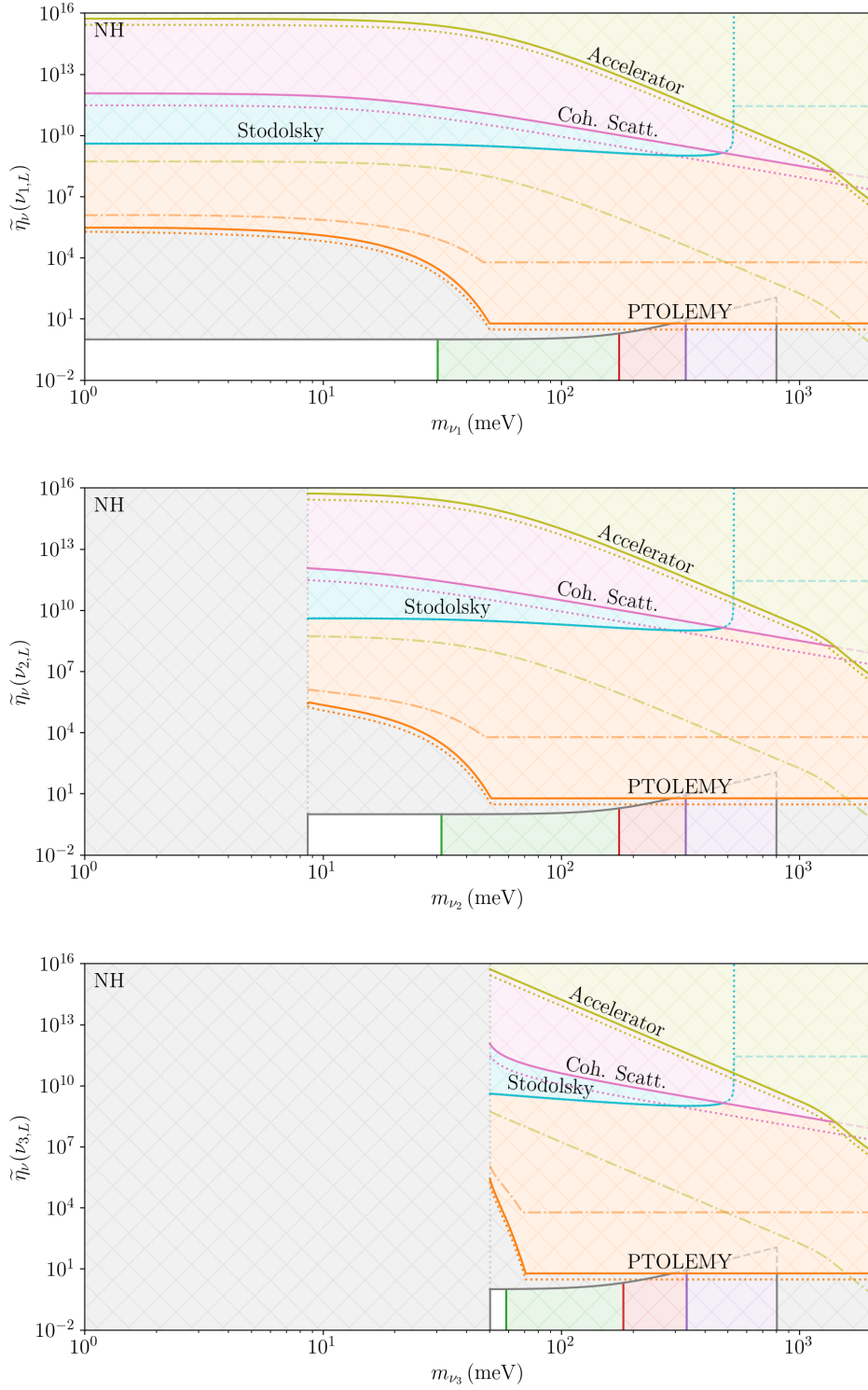
Figure 9. Sensitivity of each direct detection proposal to the CνB overdensity as a function of the neutrino mass, assuming T_{\nu_i} = T_{\nu,0} and only left (right) helicity (anti)neutrinos in the normal mass hierarchy. See the text and table 3 for a full description of the figure.
