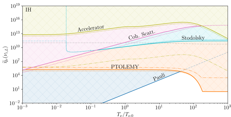
Figure 12. Sensitivity of each direct detection proposal to the C\nu B overdensity as a function of the neutrino temperature, assuming m_{\nu_3} = 10 meV and only left (right) helicity (anti)neutrinos in the inverted mass hierarchy. See the text and table 3 for a full description of the figure.
