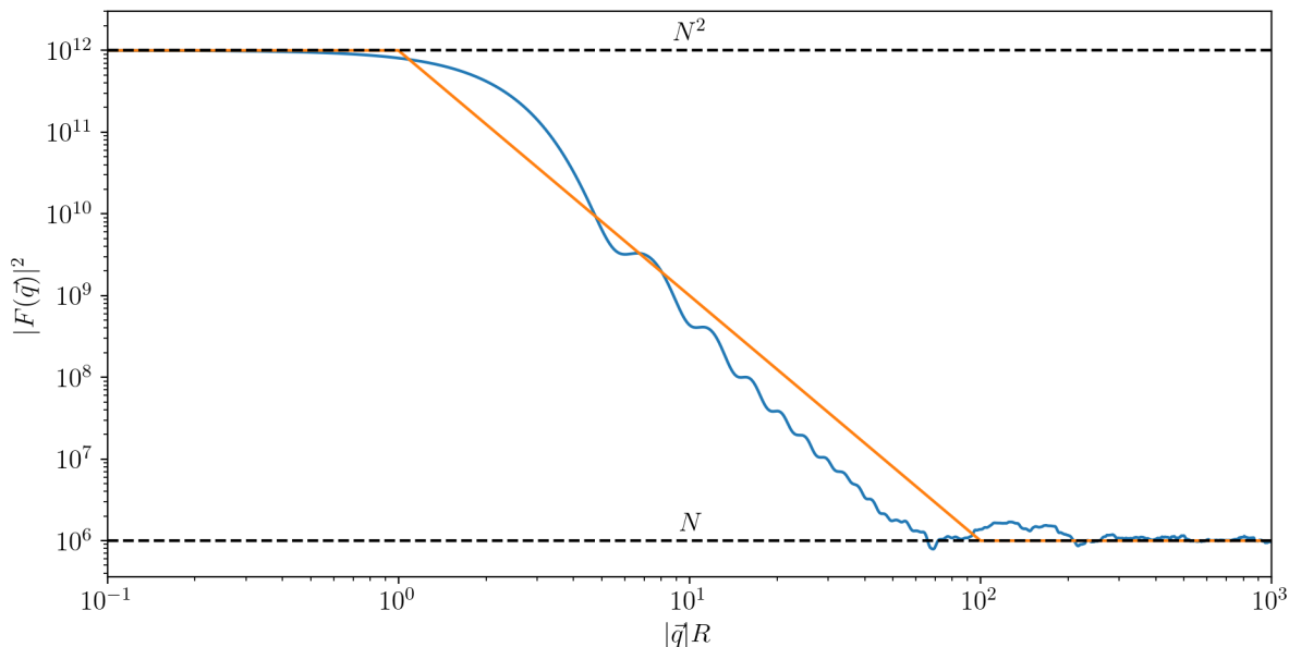
Figure 15. Structure factor for a spherical target of radius R containing N = 10^6 randomly placed scattering centres, smoothed using a moving average. For simplicity, we choose \vec{q} = (0, 0, |\vec{q}|) . The true value (D.10) is plotted in blue, whilst the approximation (D.12) is shown in orange. The wiggles in the true value at |\vec{q}|R > 1 correspond to the Bragg condition, \vec{q} \cdot (\vec{x}_i - \vec{x}_j) = n\pi for n \in \mathbb{Z} , being satisfied, where coherence is partially restored.
