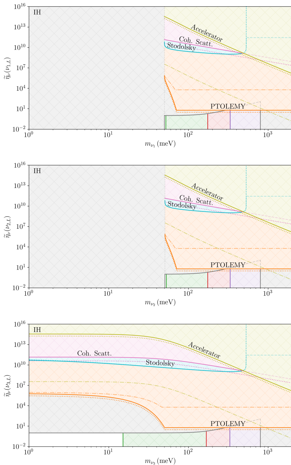
Figure 10. Sensitivity of each direct detection proposal to the C\nu B overdensity as a function of the neutrino mass, assuming T_{\nu_i} = T_{\nu,0} and only left (right) helicity (anti)neutrinos in the inverted mass hierarchy. See the text and table 3 for a full description of the figure.
