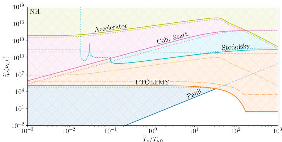
Figure 11. Sensitivity of each direct detection proposal to the C\nu B overdensity as a function of the neutrino temperature, assuming m_{\nu_1} = 10 meV and only left (right) helicity (anti)neutrinos in the normal mass hierarchy. See the text and table 3 for a full description of the figure.
