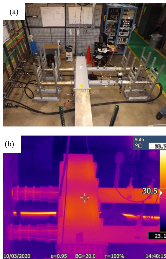
Figure 2: (a) Photo of 4-port waveguide combiner configured for high-power backfeed test, with resistive RF loads terminating all coaxial ports. (b) Infrared thermal image of the waveguide combiner at 193-kW CW input power.
