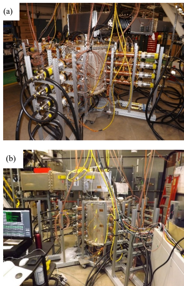
Figure 4: (a) Photo of combining cavity configured for the 200-kW backfeed test with 25-kW resistive RF loads terminating each of the sixteen coaxial ports. (b) The combining cavity configured for the combiner-mode test. Note the black coaxial cables connecting 2-kW amplifier outputs to cavity input ports.
