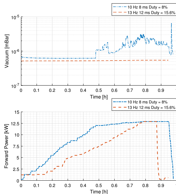
Figure 4: RF conditioning: time evolution of the vacuum pressure (top) and forward power at directional coupler of the SSPA (bottom).
