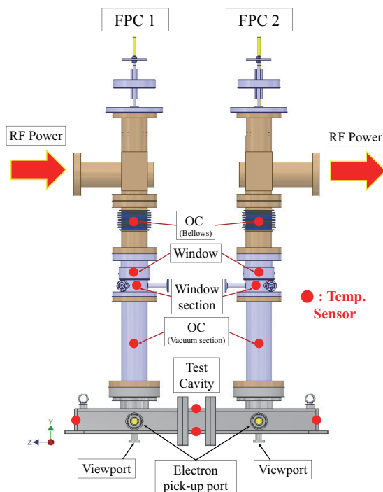
Figure 3: (a) Test bench setup of the power couplers and a test cavity and (b) geometry of a test cavity.
