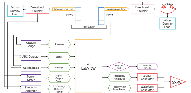
Figure 2: Test bench diagram for the high-power test of the power coupler.
