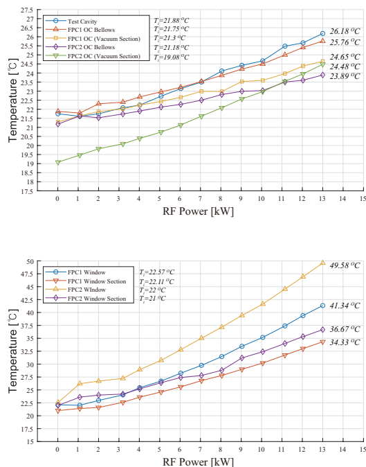
Figure 6: Temperature variation by applied RF power: (a) the test cavity (circle), FPC1 bellows at the outer conductor (triangle), FPC1 outer conductor (square), and FPC2 bellows at the outer conductor (diamond), and FPC2 outer conductor (inverted triangle); (b) the FPC1 RF window (circle), FPC1 window section (inverted triangle), FPC2 RF window (triangle), and FPC2 window section (diamond).
