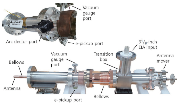
Figure 1: Manufactured model of the 325 MHz power coupler.
