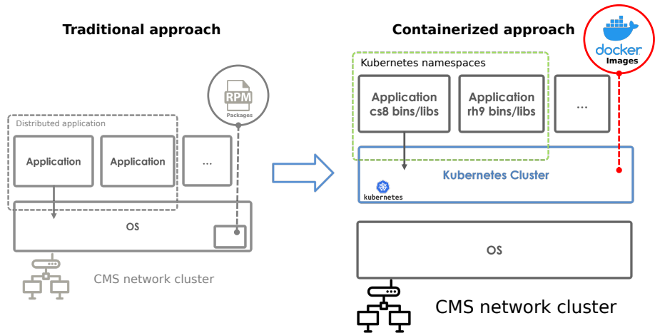
Figure 1. In traditional approach, a physical machine has libraries specific to one OS distribution installed. In containerized approach, OS distribution specific libraries are installed into container images. Containers with libraries from different OS distributions can be used on the same physical machine.
