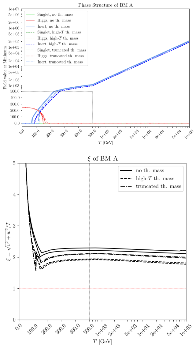
FIG. 4. Phase structure (upper panel) and EW vev-temperature ratio (lower panel) as a function of temperature, for different finite temperature implementations, for BM point A as defined in Table I
