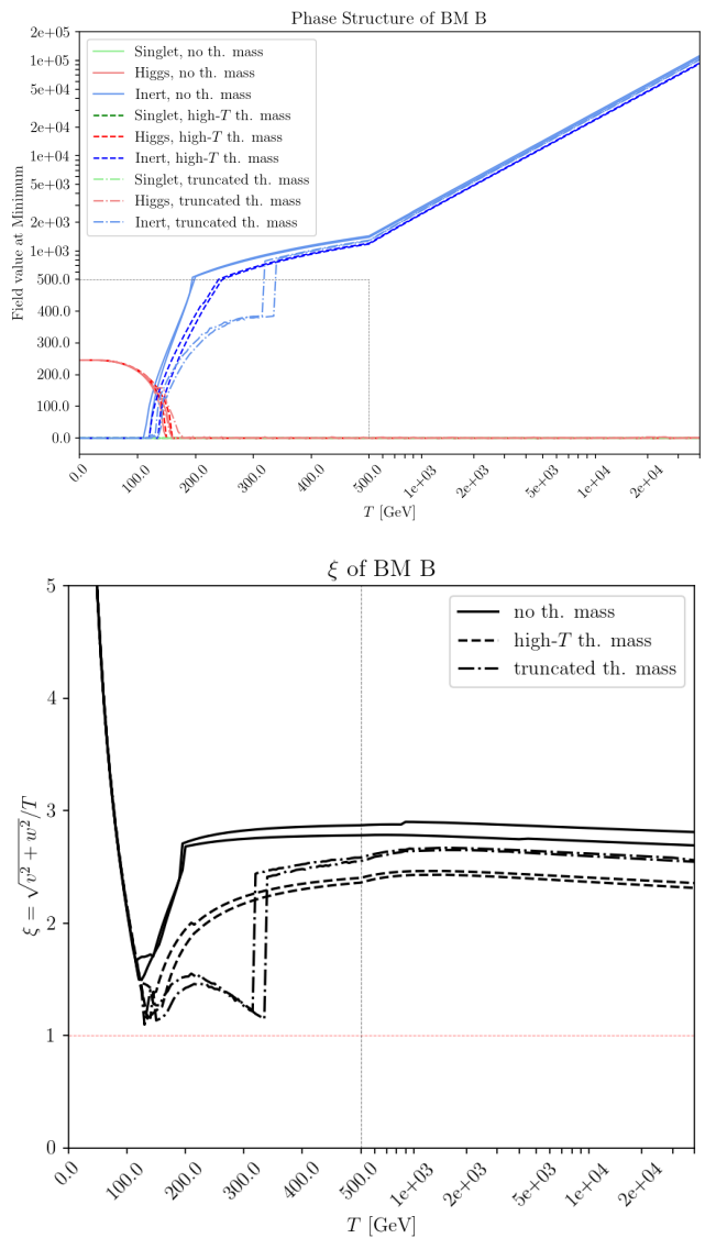
FIG. 5. Phase structure (upper panel) and EW vev-temperature ratio (lower panel) of BM B. Model parameters of the BM are given in Table I
