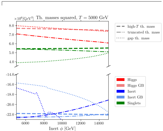
FIG. 2. Squared thermal mass of the scalars for the BM scenario B as a function of the inert field values at T = 5000 GeV for different thermal mass implementations.
