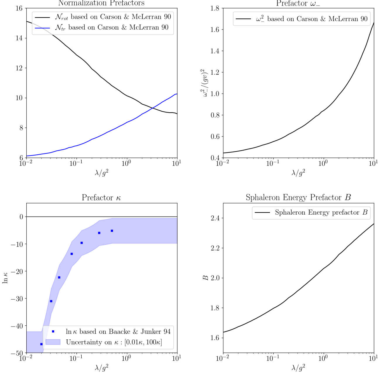
FIG. 6. Input values for the sphaleron decay rate in eq. (48). \mathcal{N}_{tr} and \mathcal{N}_{rot} are taken from [54, Fig. 5], \omega_- is taken from [54, Fig. 6], and \kappa is taken from [57], including uncertainties as explained in the text, and the energy prefactor B is computed also as discussed in the text. All quantities are plot against \lambda/g^2 , the ratio of the corresponding quartic to the gauge coupling.
