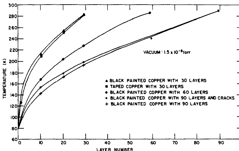
Fig. 3. Temperature distribution of MLI for various systems.
