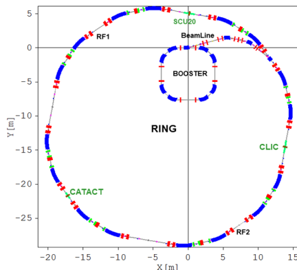
Figure 1: Model of the KARA ring [3]. The 22.5° bending magnets are depicted in blue, quadrupoles in red and the sextupoles are marked in green. The CATACT/CLIC wigglers are shown by long green strips.
