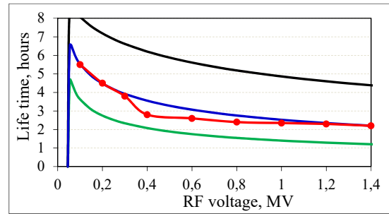
Figure 6: Beam lifetime as a function of the RF voltage at low momentum compaction optics with \alpha = +10^{-4} . Beam energy is 1.3 GeV. Black, blue and green curves correspond to computer simulations at beam current of 0.2, 0.5 and 1 mA/bunch. Measured data are marked by red curve.
