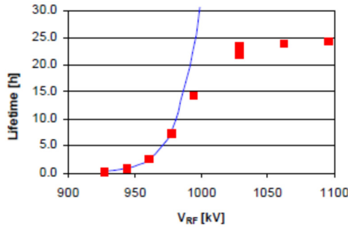
Figure 4: Beam lifetime versus RF voltage at 2.5 GeV user operation mode of KARA ring. Measured data are marked by red squares. Line is the calculated quantum lifetime at low voltage points. Figure is taken from [8].
