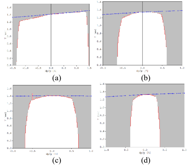
Figure 3: Off-momentum dynamic aperture of KARA ring at different operation regimes: (a) user optics with momentum compaction factor \alpha = 9 \cdot 10^{-3} ; (b) positive low- \alpha optics with \alpha = +1 \cdot 10^{-4} ; (c) negative low- \alpha operation mode with \alpha = -1.4 \cdot 10^{-4} and (d) negative- \alpha optics with \alpha = -7 \cdot 10^{-3} and dispersion stretched to \pm 1.6 m.
