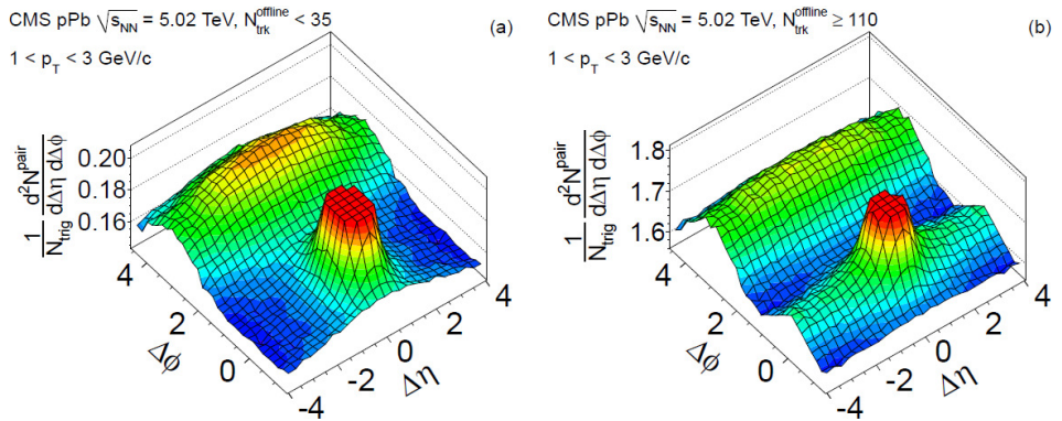
Fig. 7. Two-dimensional (2D) two-particle correlation functions for pairs of charged particles with 1 < p_T < 3 \text{ GeV}/c [24]. Results are shown (a) for low-multiplicity events ( N_{\text{trk}}^{\text{offline}} < 35 ) and (b) for a high-multiplicity selection ( N_{\text{trk}}^{\text{offline}} \geq 110 ). The sharp near-side peaks from jet correlations have been truncated to better illustrate the structure outside that region.
