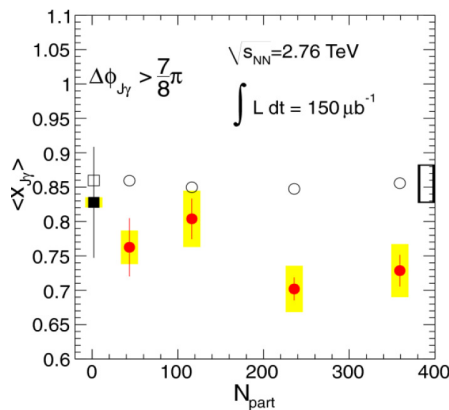
Fig. 3. (Color online) Mean values of the jet-to-photon p_T ratio as a function of the number of participant nucleons, for isolated photons of p_T^\gamma > 60 GeV/ c and jets of p_T^{\text{jet}} > 30 GeV/ c [13]. Photons were restricted to the region of |\eta| < 1.44 and jets to |\eta| < 1.6 . PbPb data are shown as red solid points, and PYTHIA+HYDJET simulations as circles. Results for pp data (black filled square) and PYTHIA- pp (open square) are also presented. Error bars and yellow boxes denote statistical and point-to-point systematic uncertainties, respectively. The empty box at the far right indicates the correlated systematic uncertainty.
