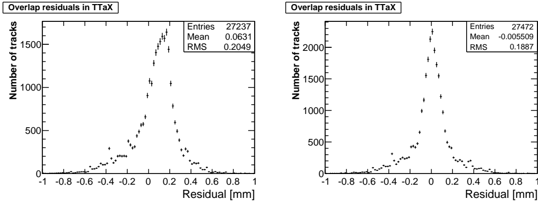
Figure 2.9: Distribution of TT residuals with alignments performed for two different periods (left and right). The same alignment constants are used for both periods, determined with data from the second period (on the right). The two periods differ by the TT operating temperature.
