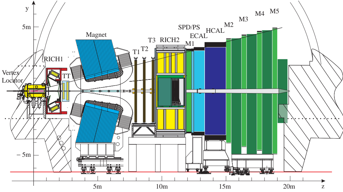
Figure 1.1: The LHCb detector.
