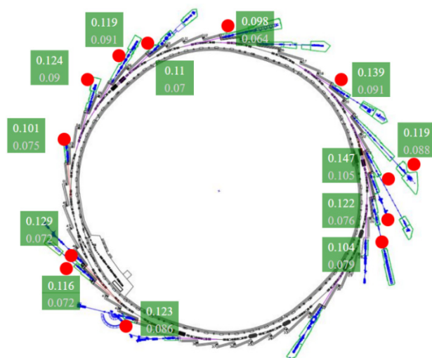
Figure 4: Positioning of monitors for TPS beamlines.
