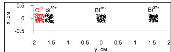
Figure 11: Bi and O ions distribution at slit CL2.
