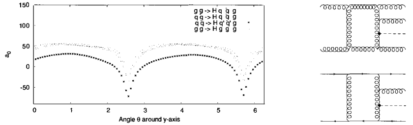
Figure 2: Left: Finite-term of the virtual matrix elements for gg \rightarrow Hq\bar{q}g (red), q\bar{q} \rightarrow Hq\bar{q}g (green), q\bar{q} \rightarrow Hq'\bar{q}'g (red), gg \rightarrow Hggg (purple). Right: sample hexagon diagrams which enter in the six-parton one-loop amplitudes for gg \rightarrow Hggg and q\bar{q} \rightarrow Hq\bar{q}g . The dot represents the effective ggH vertex.
