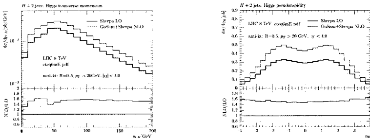
Figure 1: Transverse momentum p_T and pseudorapidity \eta of the Higgs boson, when produced in association with two jets.
