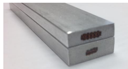
Fig. 3. DS1 and DS2 Al-stabilized cables after conforming and cold-work.
