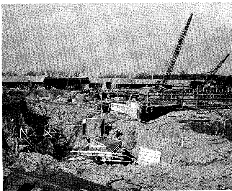
Fig. 3. The Cross Gallery. The Booster Tunnel is at the left, with the 8-GeV Transfer Tunnel in the foreground.
