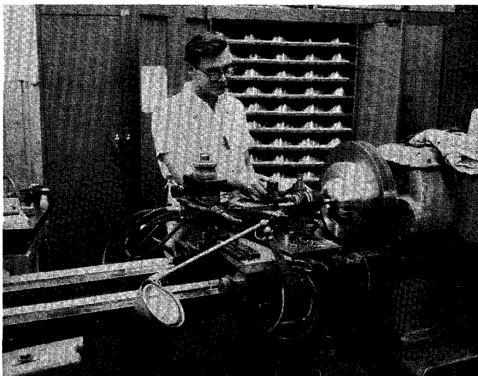
Fig. 8. Richard Gorski machining a drift-tube cap in the Linac Building. Finished caps are stored behind.
