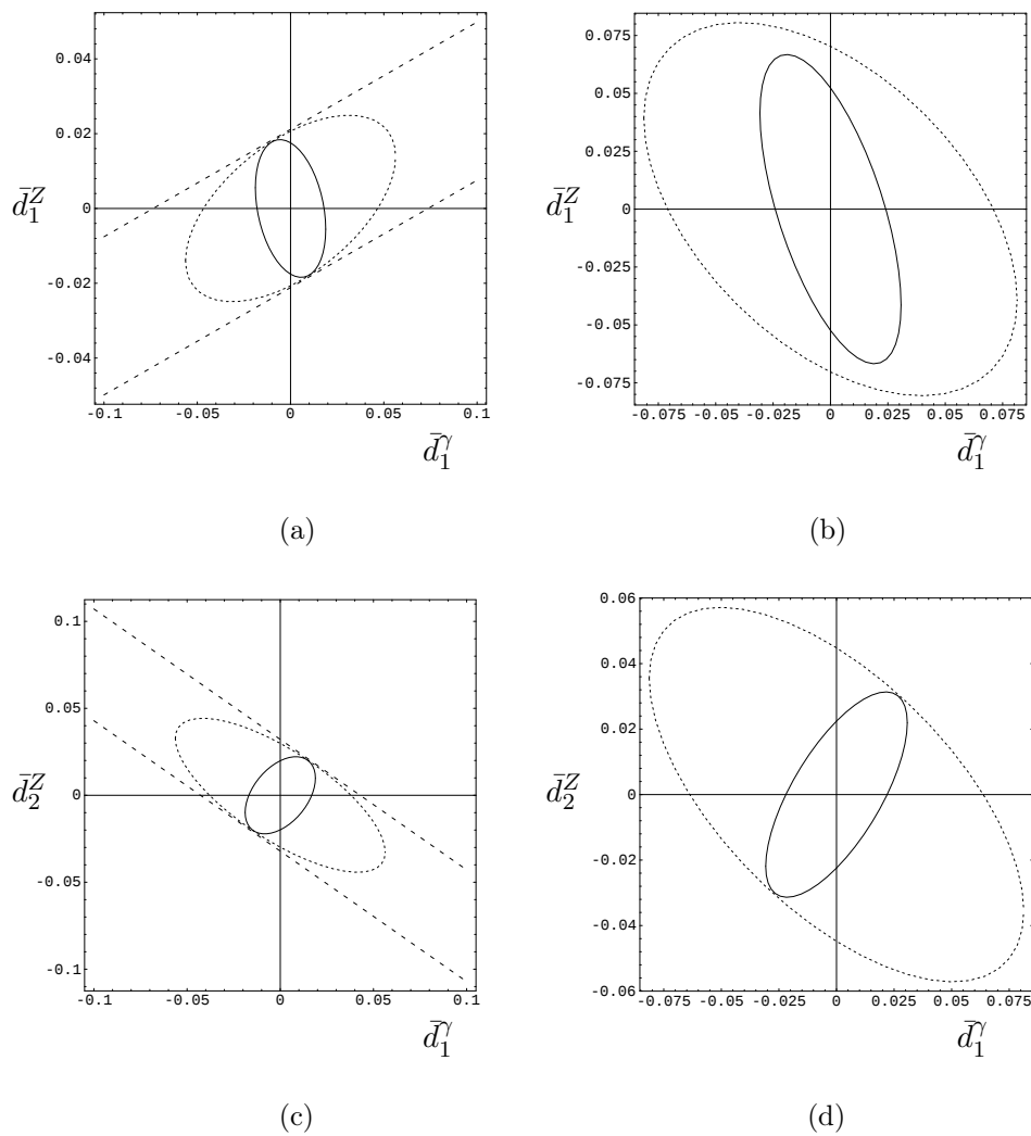
Fig. 1. Observability limits in the 6-parameter case; with polarized beams (a) (c), with unpolarized beams (b) (d); from asymmetries alone (---), from asymmetries and the 3 integrated \rho_{ij}^{L+R} matrix elements with a normalization uncertainty of 2% (.....), 20% (—).
