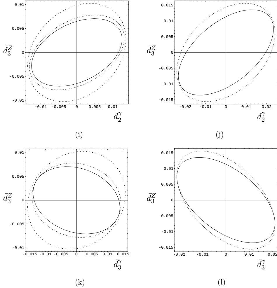
Fig. 3. Observability limits in the 6-parameter case; with polarized beams (i) (k), with unpolarized beams (j) (l); from asymmetries alone (---), from asymmetries and the 3 integrated \rho_{ij}^{L+R} matrix elements with a normalization uncertainty of 2% (.....), 20% (—).
