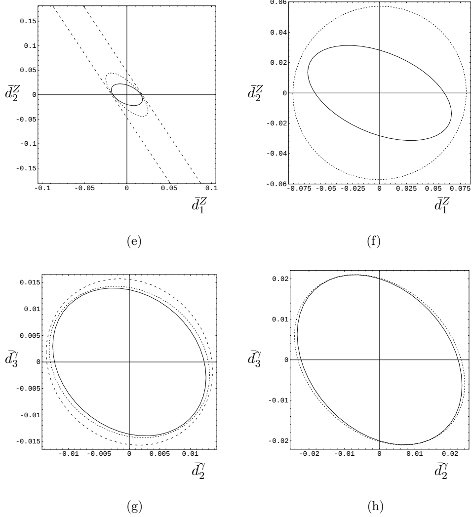
Fig. 2. Observability limits in the 6-parameter case; with polarized beams (e) (g), with unpolarized beams (f) (h); from asymmetries alone (---), from asymmetries and the 3 integrated \rho_{ij}^{L+R} matrix elements with a normalization uncertainty of 2% (.....), 20% (—).
