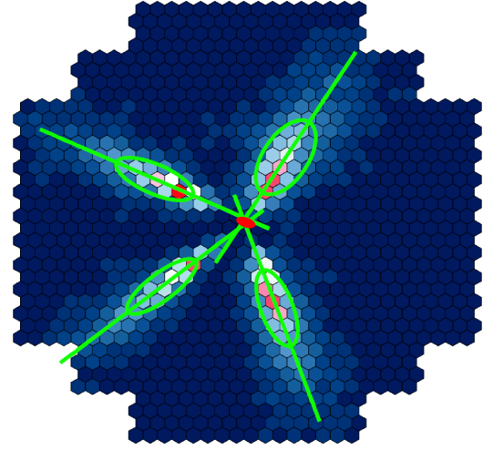
(b) Superimposed camera image of an event seen by the four H.E.S.S. I type telescopes. The Hillas ellipses and the shower direction in each camera are shown in light green. The intersection of the different major axes of all ellipses is the source position in the Nominal System.
