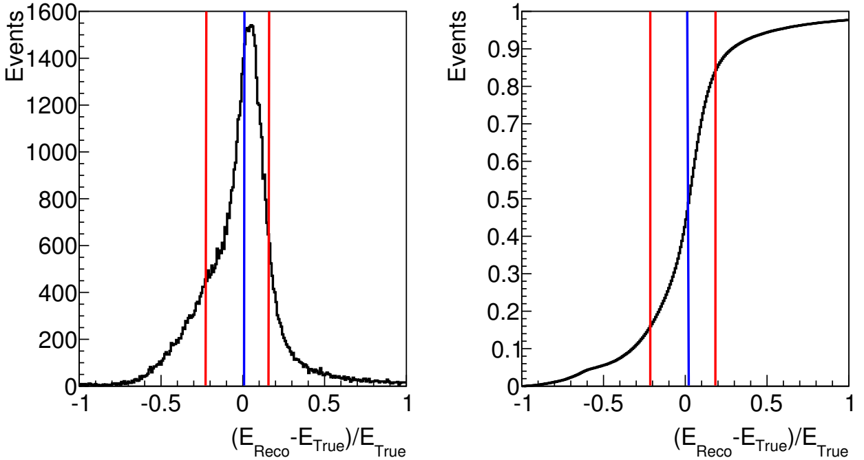
Figure 4.29.: Distribution of the energy offset \Delta_E for an exemplary energy bin on the left and the cumulative distribution on the right. The blue line indicates the median of the distribution which is called energy bias and the two red lines indicate the 68 % containment radius around the median. The average of the two radii is called energy resolution.
