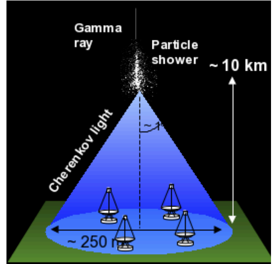
(b) A gamma-ray induced air shower at a height of maximum emission of \approx 10 km with its resulting cone of Cherenkov light with an opening angle of \approx 1^\circ (not to scale). Multiple telescopes are placed within the pool of Cherenkov light on the ground for stereoscopic observation.
