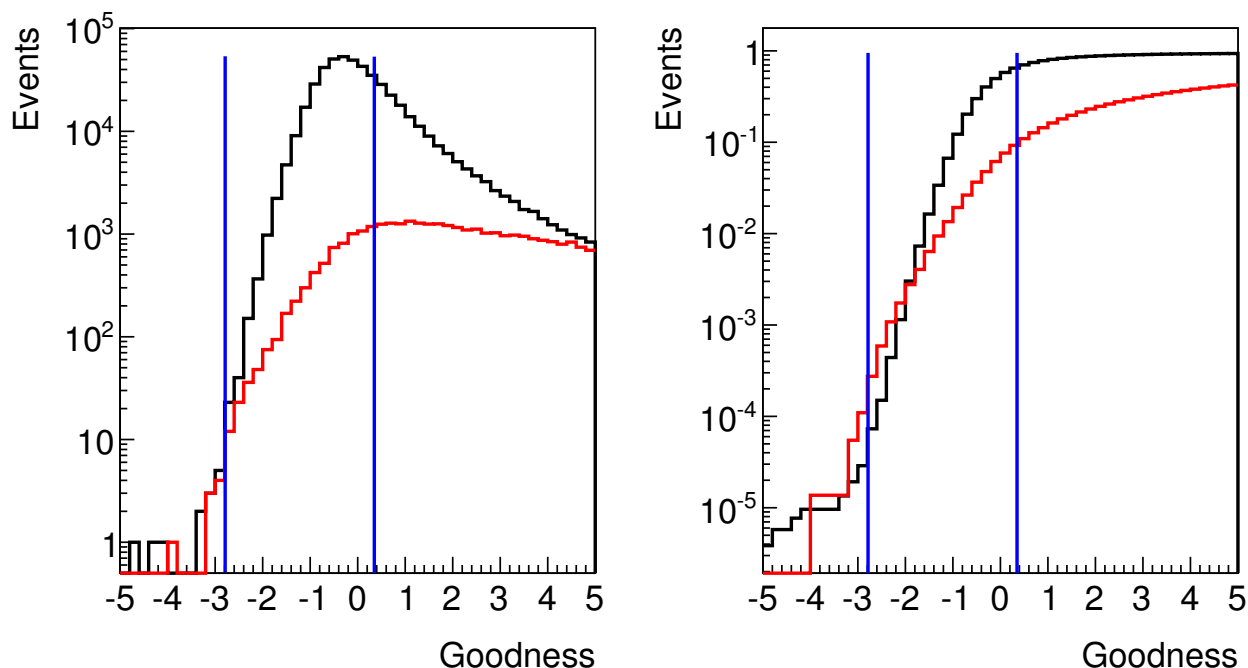
Figure 4.25.: Exemplary gamma-ray (black) and proton distribution (red) of the Mean Reduced Scaled Goodness for the energy bin around 2.1 TeV and the corresponding cumulative distribution. The minimum and maximum cut value are indicated by the vertical blue lines. The fraction of events surviving the cut can be easily obtained using the cumulative distributions.
