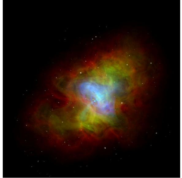
(b) Composite image of the Crab Nebula in different energy bands. Radio in red, optical in green and X-ray in blue. The size of the Nebula is clearly inverse proportional to the energy of the radiation. Figure taken from [19].
