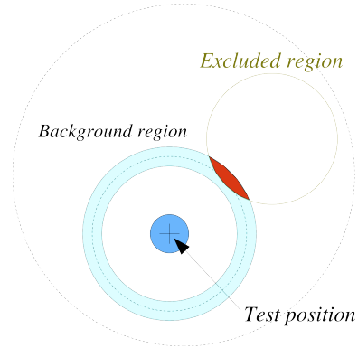
(b) Schematic of the Ring Background subtraction technique. The source region is surrounded by an annular background region. Regions containing sources of known VHE gamma-ray radiation are excluded.
