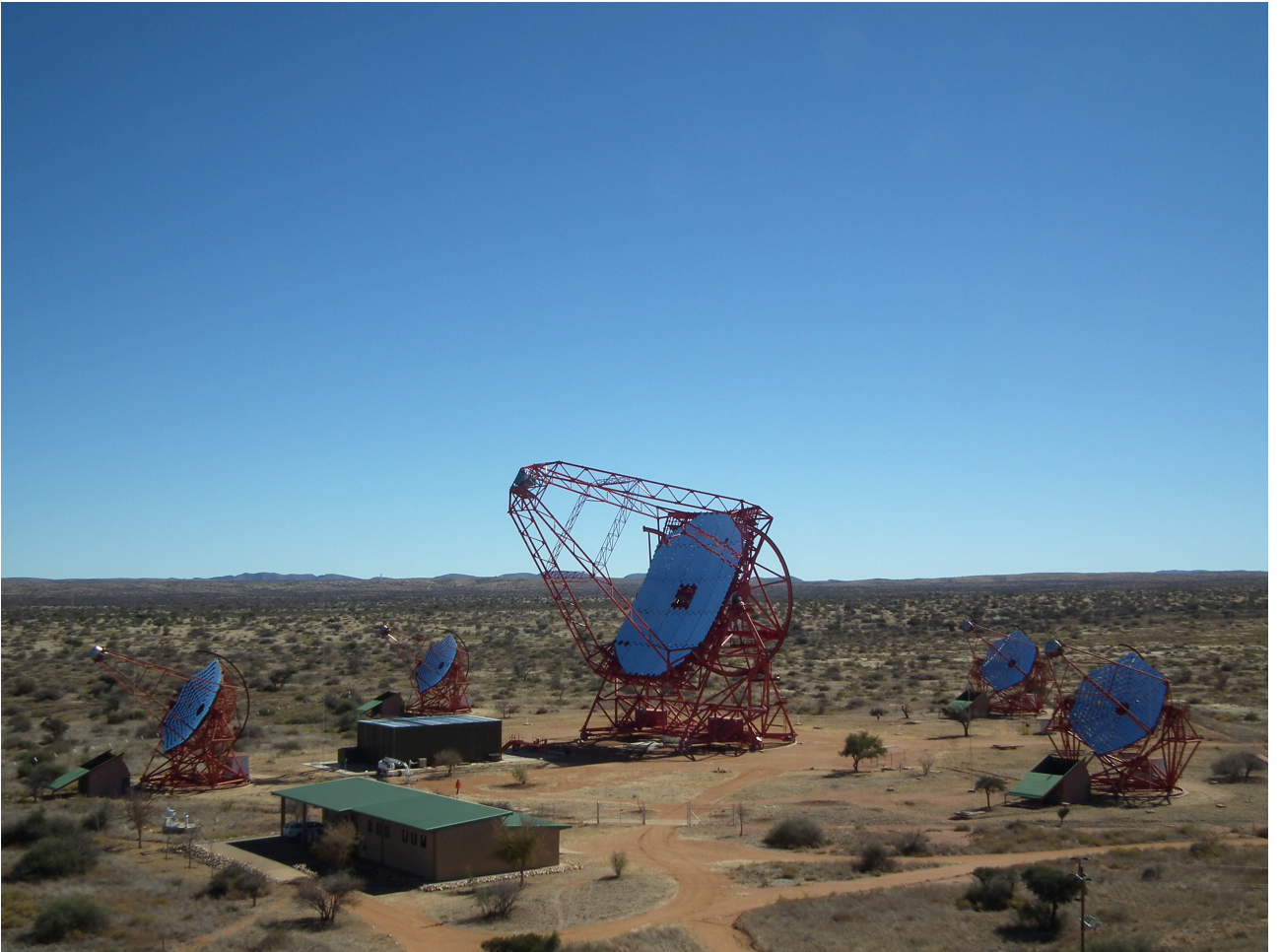
Figure 3.6.: Picture of the H.E.S.S. site in Namibia. The telescopes from right to left are CT1, CT2, CT3, and CT4. The building in the front houses the central computing farm as well as the central control room of the array.
