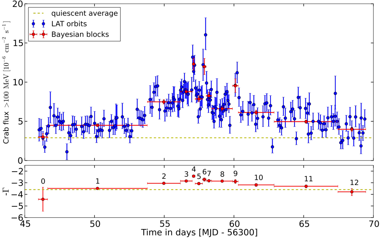
Figure 5.2.: Red data points correspond to the total Crab flux levels derived using the Bayesian block method in the upper plot whereas blue points show the orbit-binned light curve. The bottom panel shows the time evolution of the spectral index of the synchrotron component of the corresponding Bayesian blocks in the upper figure with respect to the all-time average spectral index of the synchrotron component of the Crab Nebula. Figure taken from [95].
