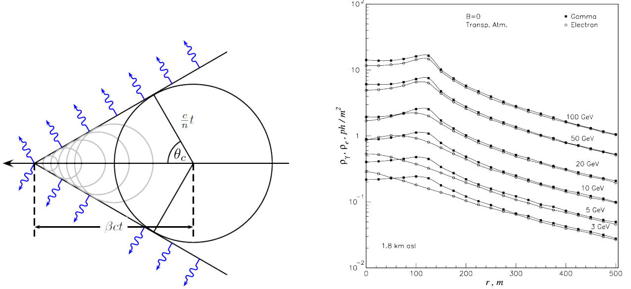
(a) Shock front of Cherenkov light (blue lines) created by a particle traveling with a speed \beta = \frac{v_p}{c} greater than the speed of light in the medium \frac{c}{n} with a refractive index n . The particle induces dipoles which upon relaxation emit spherical waves that interfere constructively forming the Cherenkov cone of light. The characteristic opening angle \theta_c and its dependence of n and \beta are shown. Figure taken from [142].
