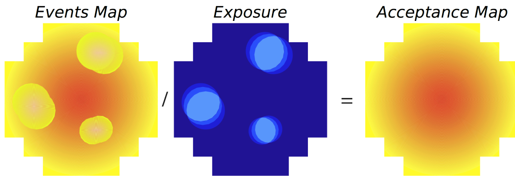
(b) The acceptance map is calculated by simple division of the summed up events and exposure maps.
