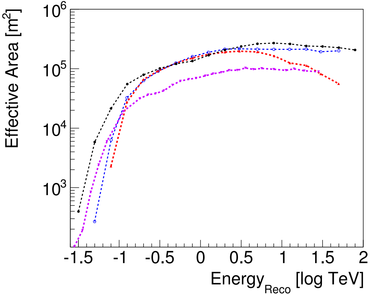
Figure 4.33.: Effective areas for the different phases of the H.E.S.S. experiment. The red and blue lines correspond to the effective area for H.E.S.S. Phase I, the former for the original Model Analysis and the latter for a Hillas analysis (both curves taken from [136]). The black line indicates the effective area for the reconstruction described in this work. The purple line shows the corresponding curve of the MAGIC II array [204].
