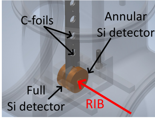
FIG. 3. Schematic view of the ASET: the silicon annular detector is placed in front of the ladder, and the silicon full detector at the back, with the RIB coming in from the front.
