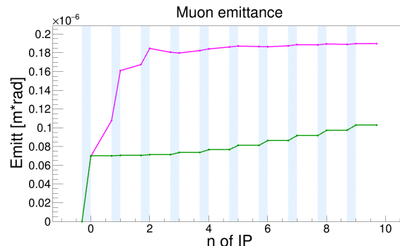
Figure 2: Comparison of \mu emittance growth in the Multiple (magenta) and Single (green) IP schemes, as a function of the target number (0 to 9). \sigma_{e^+}=150 \mu\text{m} in both cases.
