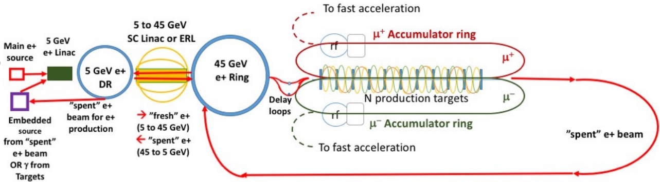
Figure 1: Layout of Scheme III for \mu production via 45 GeV e^+ beam.
