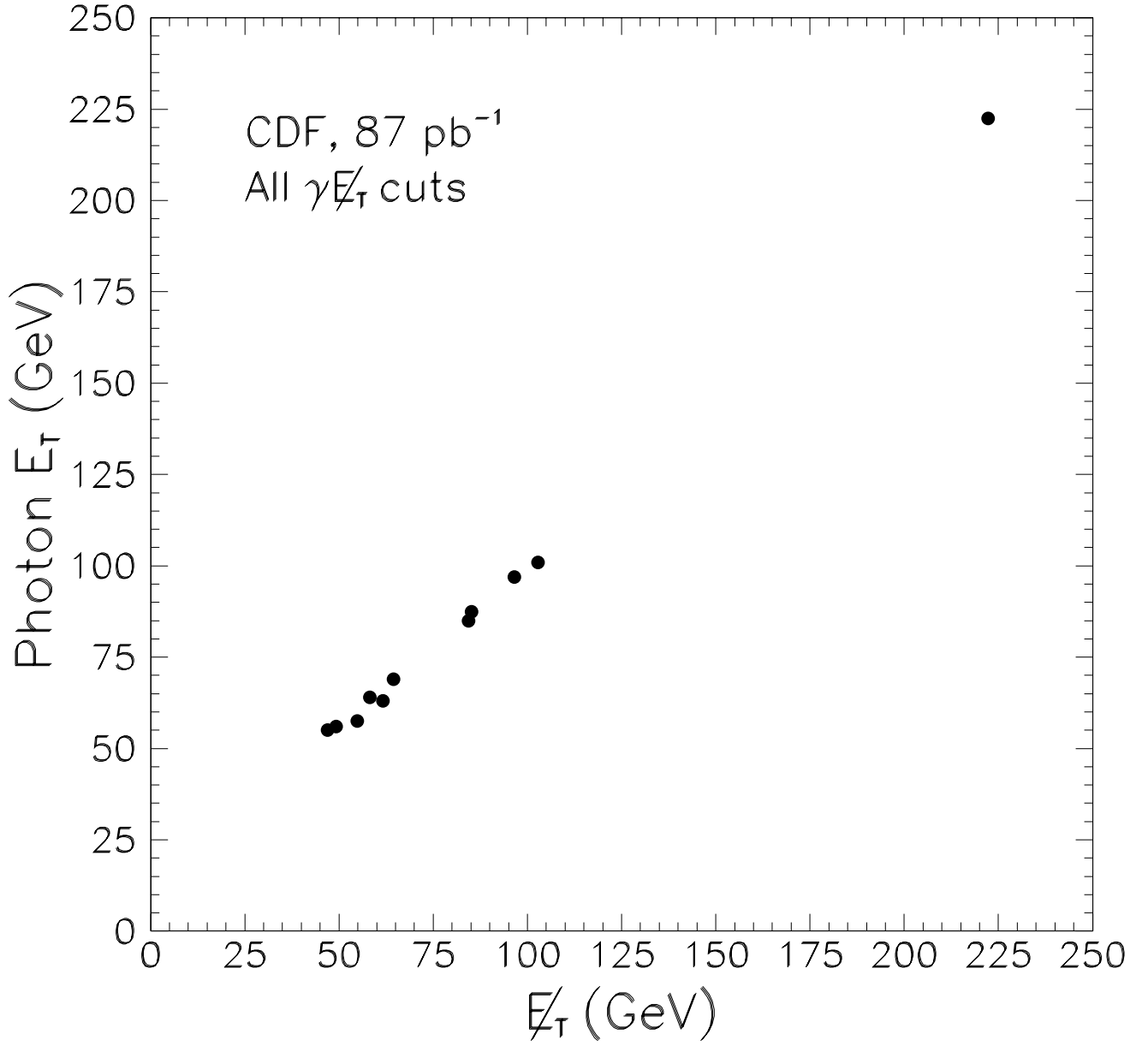
FIG. 2: Photon E_T versus E_T for the 11 events passing the selection criteria. The tight correlation of E_T^\gamma and E_T reflects the detector resolution for unclustered energy.
