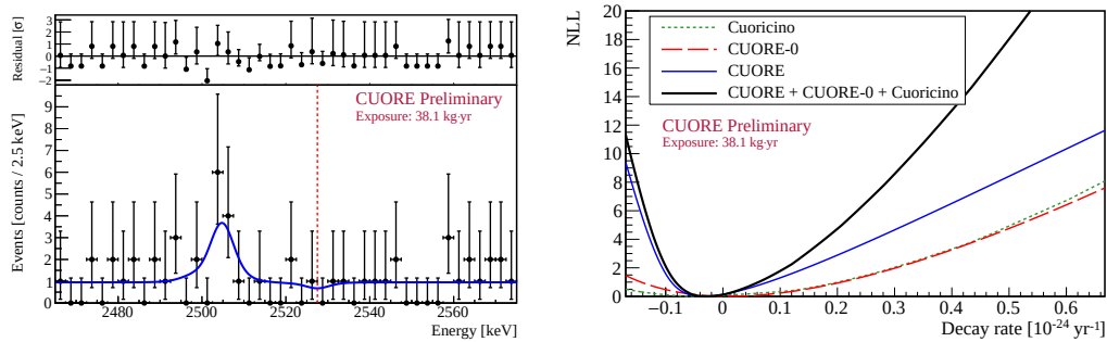
Figure 4. Left: Best-fit model from the UEMF fit (solid blue line) overlaid on the spectrum of \beta\beta(0\nu) decay candidates observed in CUORE. The peak near 2500 keV is attributed to ^{60}\text{Co} [16]. Right: Profile negative-log-likelihood curves for CUORE, CUORE-0, Cuoricino, and their combination..
