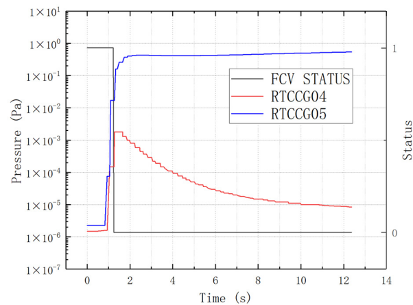
Figure 6: Response curve of the fast closing valve and the relevant vacuum gauge in Section IV when it is subjected to an unexpected airborne impact.
