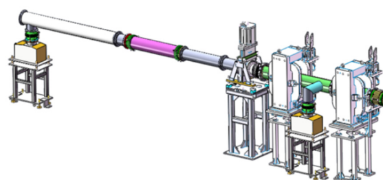
Figure 3: Partial assembly diagram of the RTBT.
