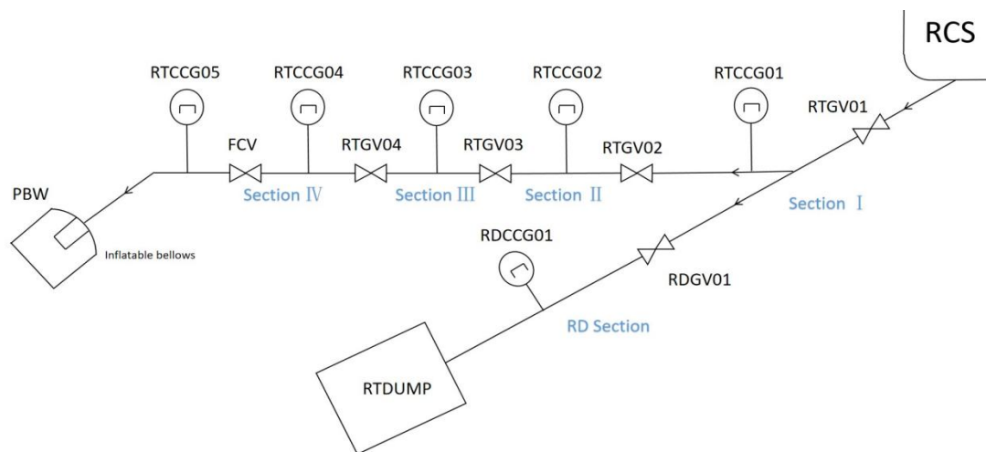
Figure 1: Section of the RTBT (RT: abbreviation of RTBT; GV: gate valve; FCV: fast closing valve).
