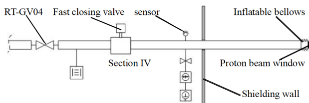
Figure 5: Schematic diagram of fast closing valve system.
