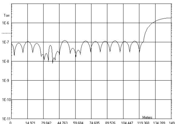
Figure 2: Pressure profile of the RTBT.
