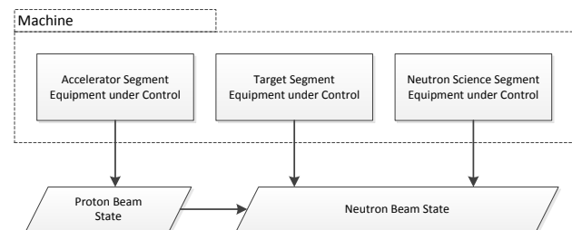
Figure 1: Simplified representation of the “machine”. Equipment under control from the accelerator segment controls the proton beam state. The neutron beam state is controlled by the Target and Neutron Science Segment EUC and is influenced by the proton beam.
