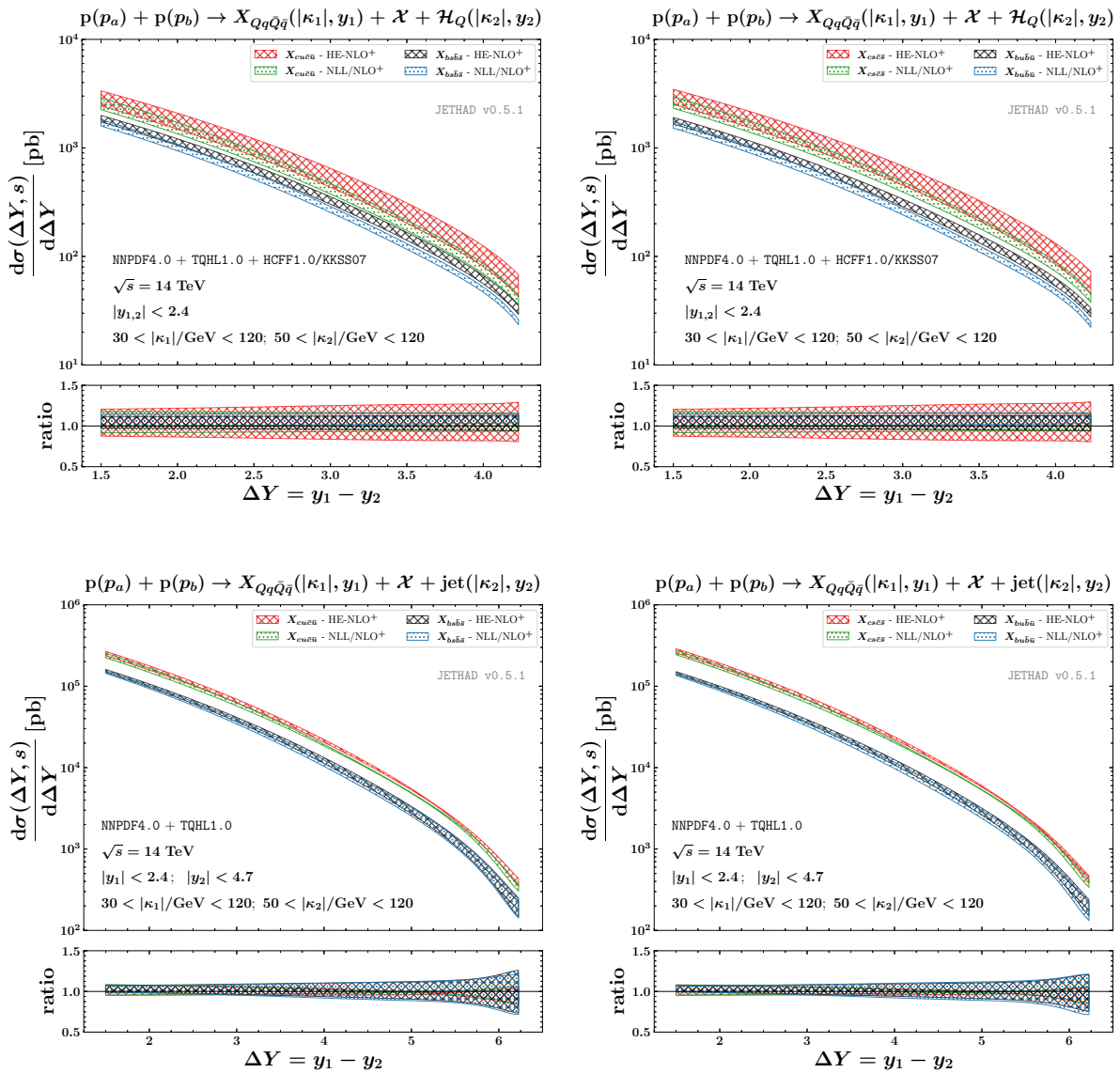
Figure 6. NLL/NLO + versus HE-NLO + \Delta Y -rates for X_{Qq\bar{Q}\bar{q}} + \mathcal{H}_Q (upper) and X_{Qq\bar{Q}\bar{q}} + \text{jet} (lower) reactions at 14 TeV LHC. Uncertainty bands are for the combined effect of MHOUs and errors on numeric integrations.
