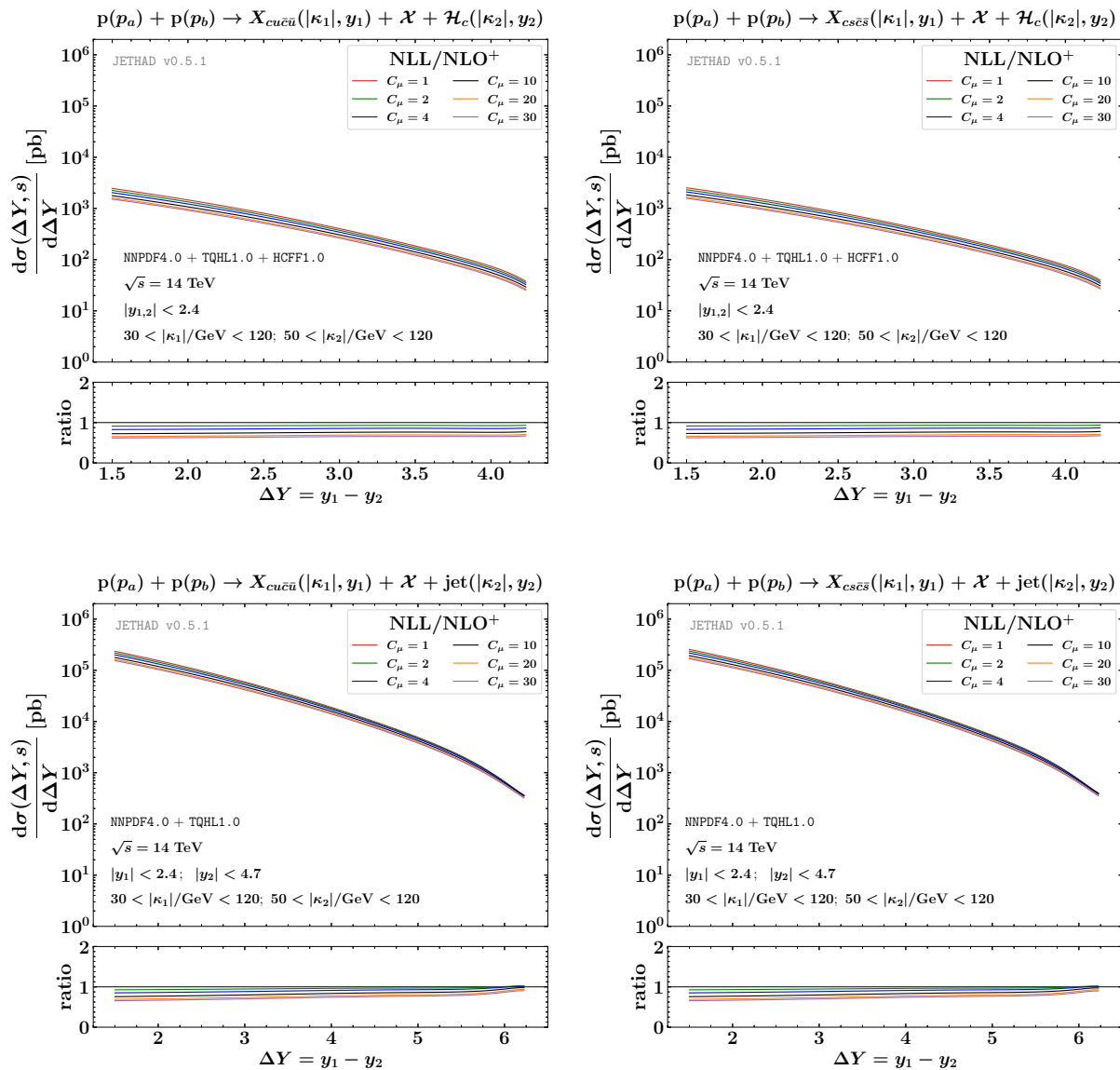
Figure 4. NLL/NLO + versus HE-NLO + \Delta Y -rates for X_{cq\bar{c}\bar{q}} + \mathcal{H}_Q (upper) and X_{cq\bar{c}\bar{q}} + \text{jet} (lower) reactions at 14 TeV LHC. An extended study of MHOUs in the range 1 < C_\mu < 30 is illustrated.
