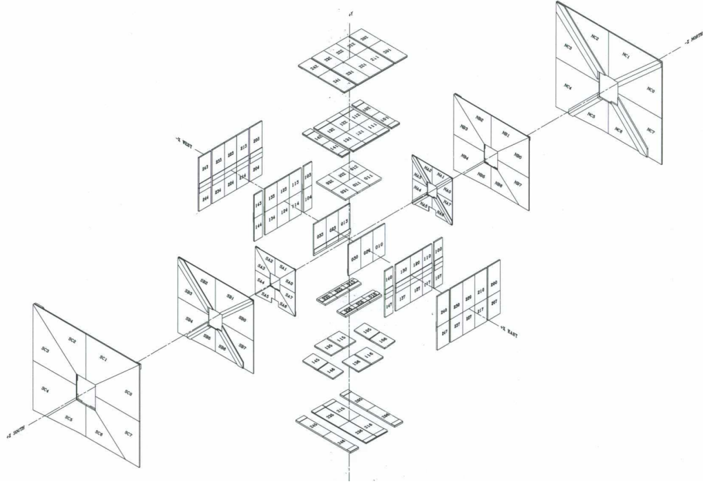
Fig. 3.21. 3-dimensional layout of the muon tracking system.
