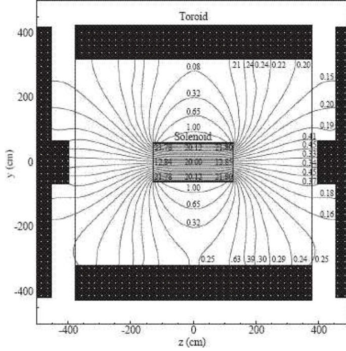
Fig. 3.19. Solenoid magnetic field in the y - z plane of the detector (in kG, 10 \text{ kG} = 1 \text{ T} ).
