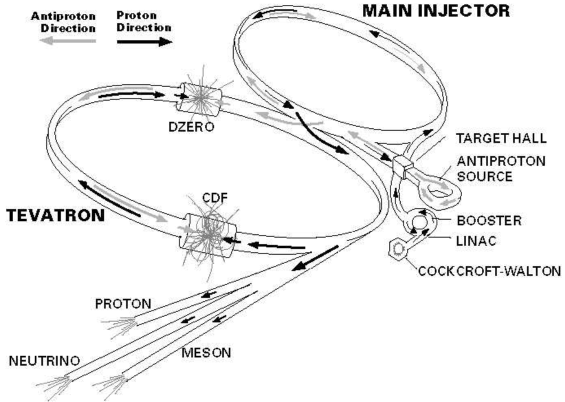
Fig. 3.1. Overview of Fermilab accelerator complex
