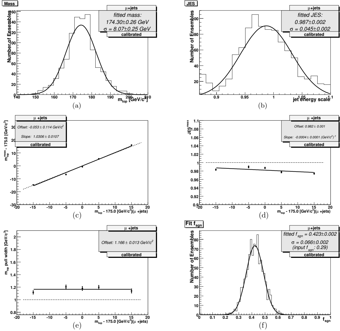
Fig. 6.22. Results of ensemble testing for ensembles with normal background fraction, heavy-flavor background and QCD included , \mu +jets (calibrated), input mass 175 GeV/c 2 ( \mu +jets): (a) output m_{top} , (b) output JES, (c) output mass vs. input mass, (d) output JES vs. input mass, (e) m_{top} pull vs. input mass, and (f) output f_{top} ,
