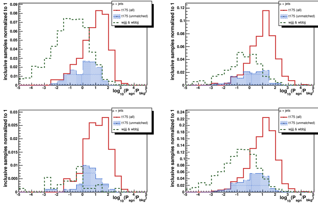
Fig. 5.8. Signal vs. background probabilities for top, Wjjjj , and Wbbjj MC events, \mu+\text{jets} (0, 1, \geq 2 tags, and all-inclusive).
