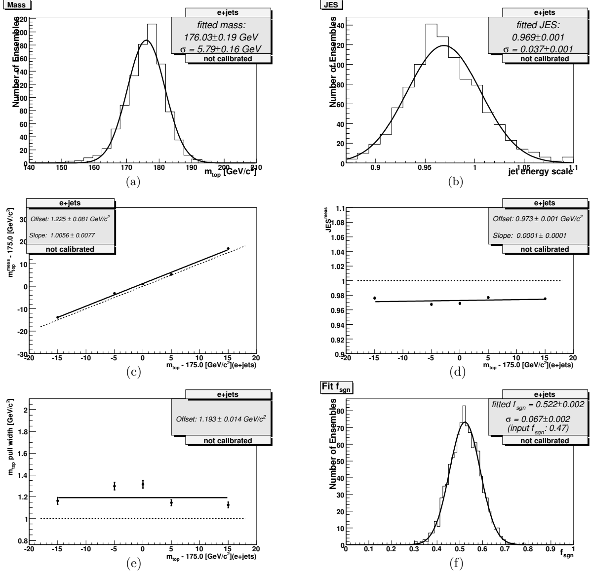
Fig. 6.7. Results of ensemble testing for ensembles with normal background fraction, heavy-flavor background included , input mass 175 GeV/c 2 (e+jets): (a) output m_{top} , (b) output JES, (c) output mass vs. input mass, (d) output JES vs. input mass, (e) m_{top} pull vs. input mass, and (f) output f_{top} ,
