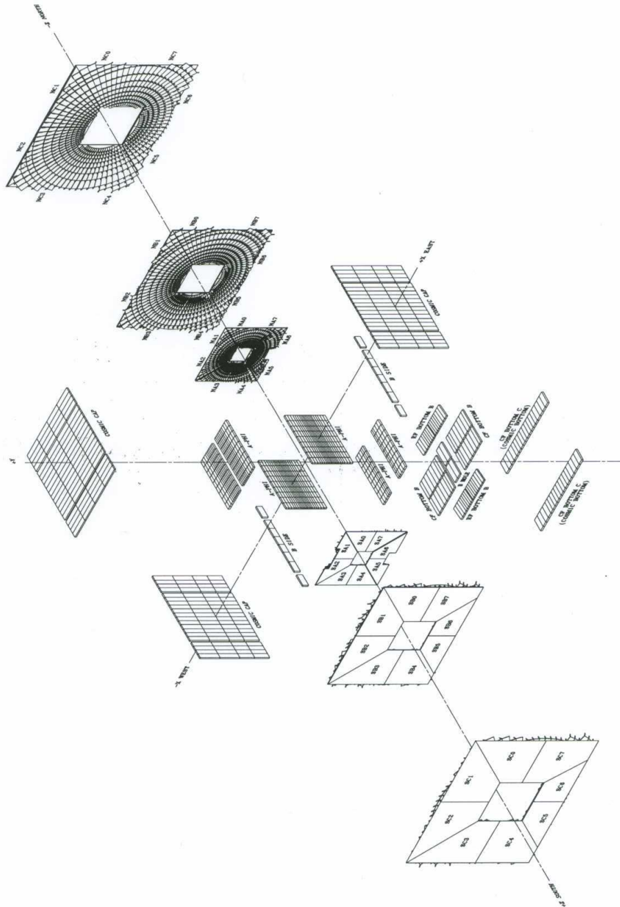
Fig. F.1. 3-dimensional layout of the muon scintillator detection system.
