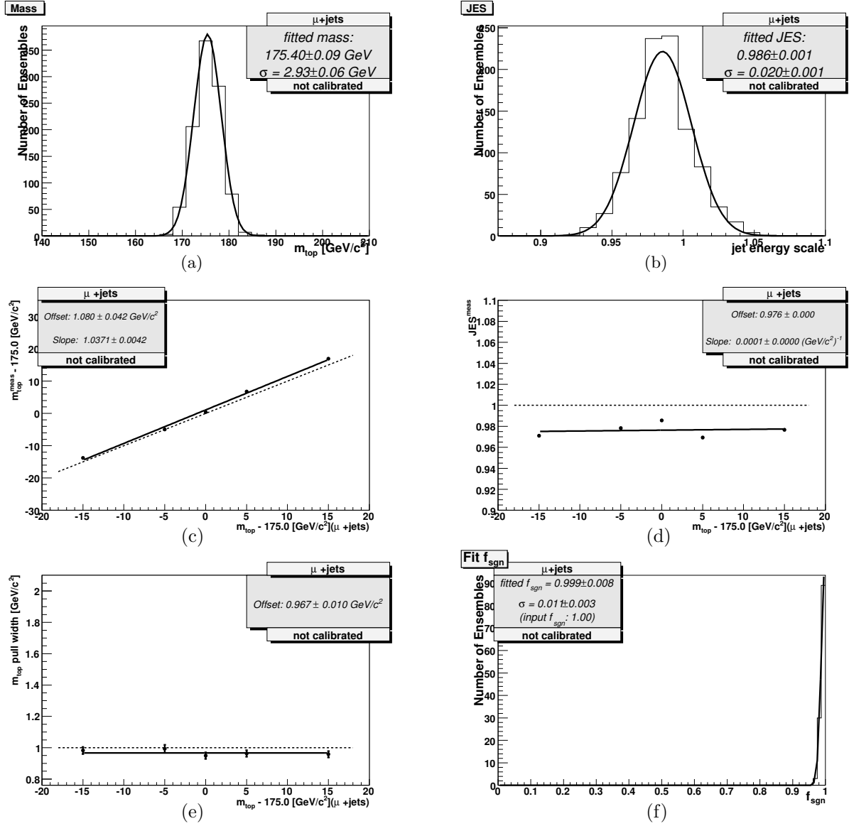
Fig. 6.2. Results of ensemble testing for signal-only ensembles ( f_{top}=1.0 ), with jet-parton matching , input mass 175 GeV/c 2 ( \mu +jets): (a) output m_{top} , (b) output JES, (c) output mass vs. input mass, (d) output JES vs. input mass, (e) m_{top} pull vs. input mass, and (f) output f_{top} ,
