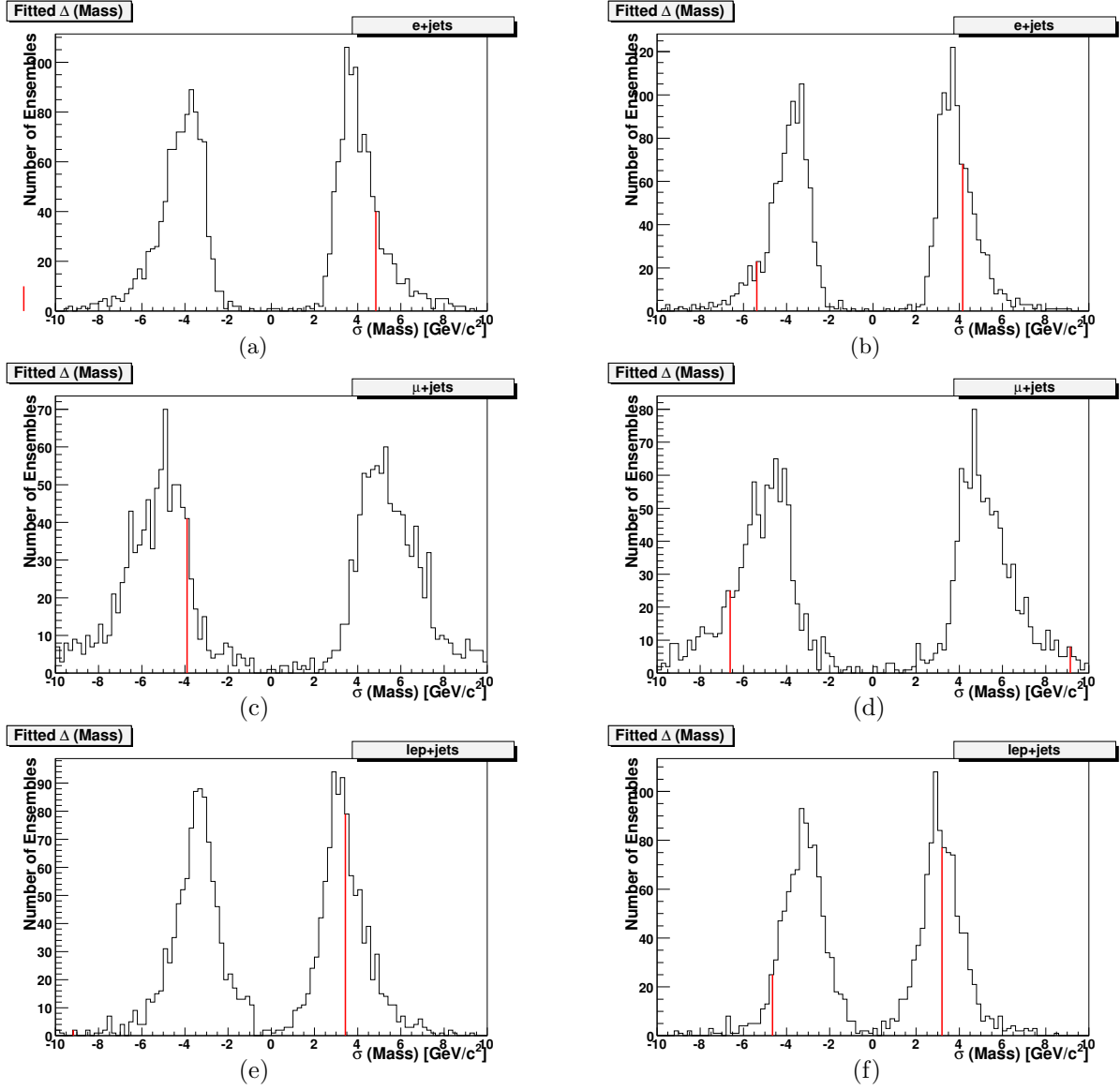
Fig. 6.39. Actual errors from data (vertical lines) and error distribution from ensemble testing, untagged ( left ) and b -tagged( right ), e+jets ( top ), \mu+jets ( middle ), and l+jets ( bottom )
