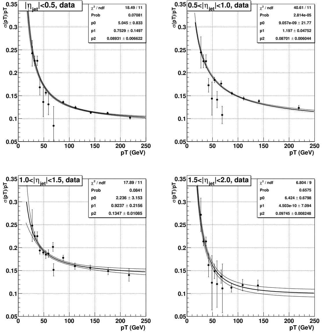
Fig. 4.5. Jet p_T resolutions for different \eta_{\text{det}} regions in data. The points below \sim 50 GeV are obtained using photon+jet events, whereas for p_T > 50 GeV resolutions are measured using dijet data. Bands of \pm 1\sigma statistical error are also shown.
