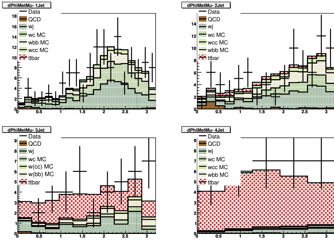
Fig. A.19. \mu +jets: \Delta\phi(\mu\text{on}, \text{missing } E_T) .
