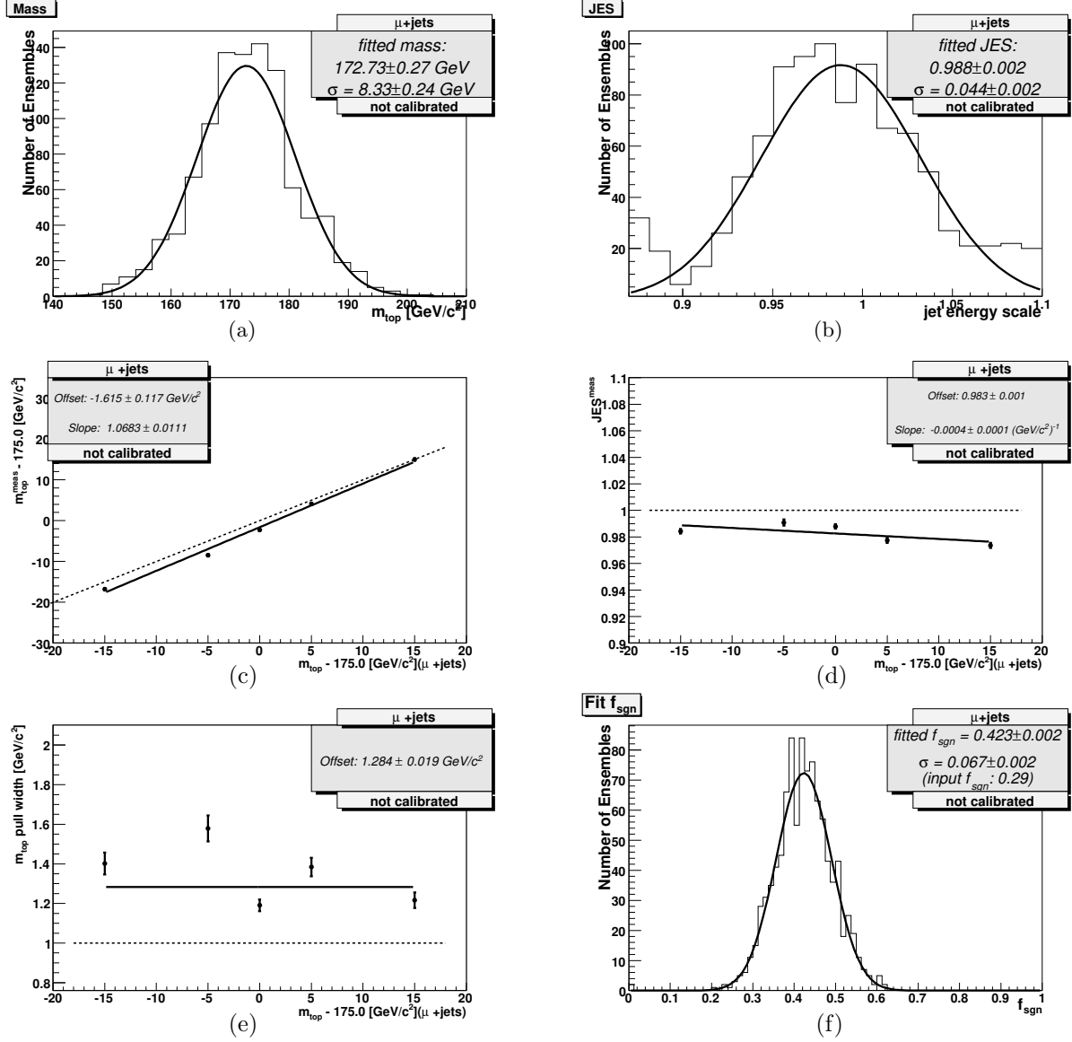
Fig. 6.10. Results of ensemble testing for ensembles with normal background fraction, heavy-flavor background and QCD included , input mass 175 GeV/c 2 (μ+jets): (a) output m_{top} , (b) output JES, (c) output mass vs. input mass, (d) output JES vs. input mass, (e) m_{top} pull vs. input mass, and (f) output f_{top} ,
