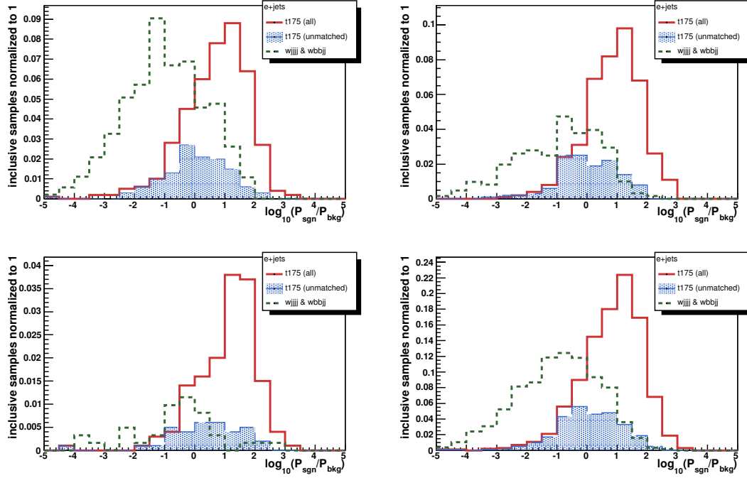
Fig. 5.7. Signal vs. background probabilities for top, Wjjjj , and Wbbjj MC events, e+\text{jets} (0, 1, \geq 2 tags, and all-inclusive).
