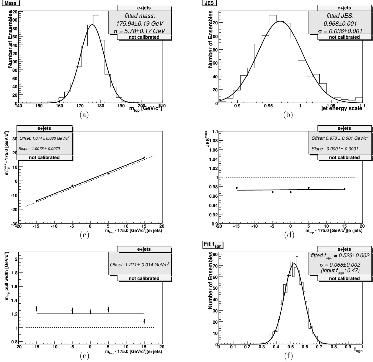
Fig. 6.5. Results of ensemble testing for ensembles with normal background fraction, all Wjjjj background , input mass 175 \text{ GeV}/c^2 ( e+jets ): (a) output m_{top} , (b) output JES, (c) output mass vs. input mass, (d) output JES vs. input mass, (e) m_{top} pull vs. input mass, and (f) output f_{sgn} ,
