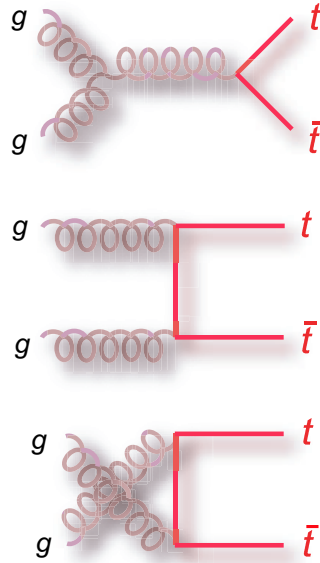
Fig. 2.2. Feynman diagrams for gg \rightarrow t\bar{t}
