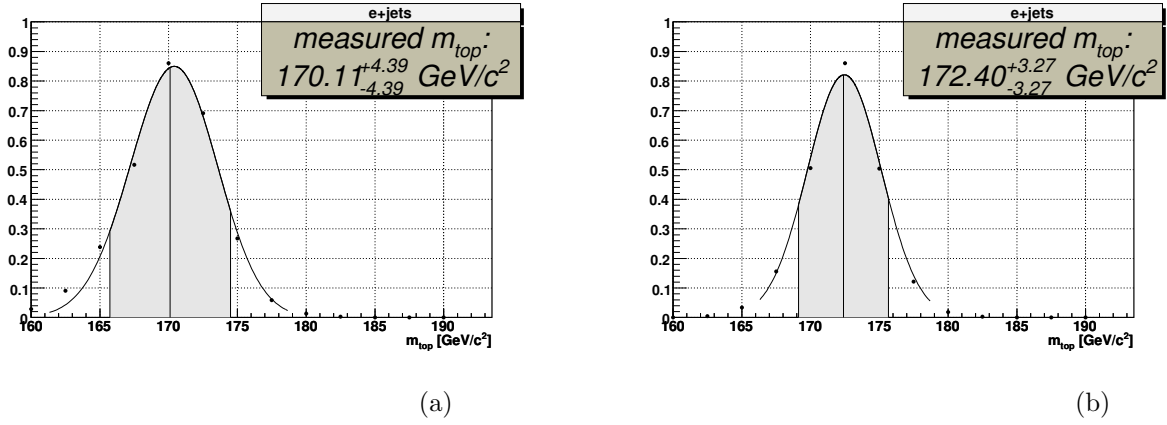
Fig. 6.35. -\ln L(m_{top}) for e+jets data events with JES fixed at 1.0, (a) without b -tagging, and (b) with b -tagging applied.
