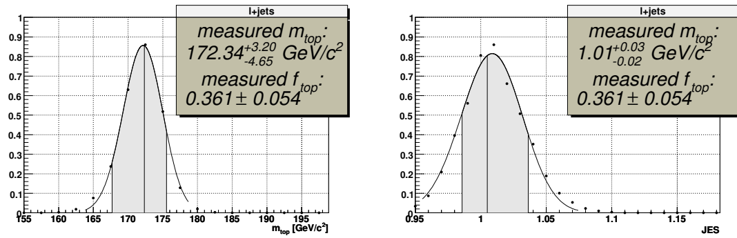
Fig. 6.32. Projection onto JES axis of -\ln L_{2D}(m_{top}, JES) for lepton+jets data events, B-TAGGING APPLIED ( e +jets and \mu +jets combined).
