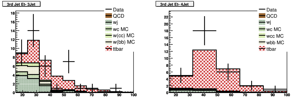
Fig. A.18. \mu +jets: 3rd leading jet p_T .
