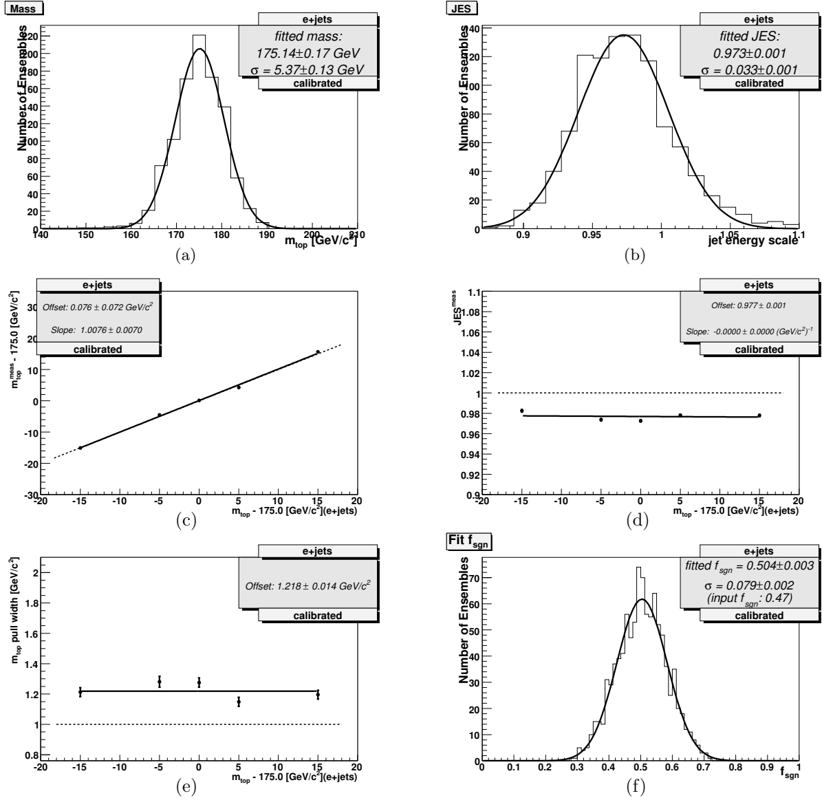
Fig. 6.24. Results of ensemble testing for ensembles with normal background fraction, heavy-flavor background and QCD included, b -tagging applied, e+jets (calibrated) , input mass 175 GeV/c 2 (e+jets): (a) output m_{top} , (b) output JES, (c) output mass vs. input mass, (d) output JES vs. input mass, (e) m_{top} pull vs. input mass, and (f) output f_{top} ,
