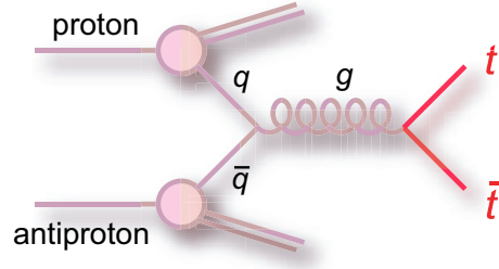
Fig. 2.1. Feynman diagram for p\bar{p} \rightarrow q\bar{q} \rightarrow t\bar{t}
