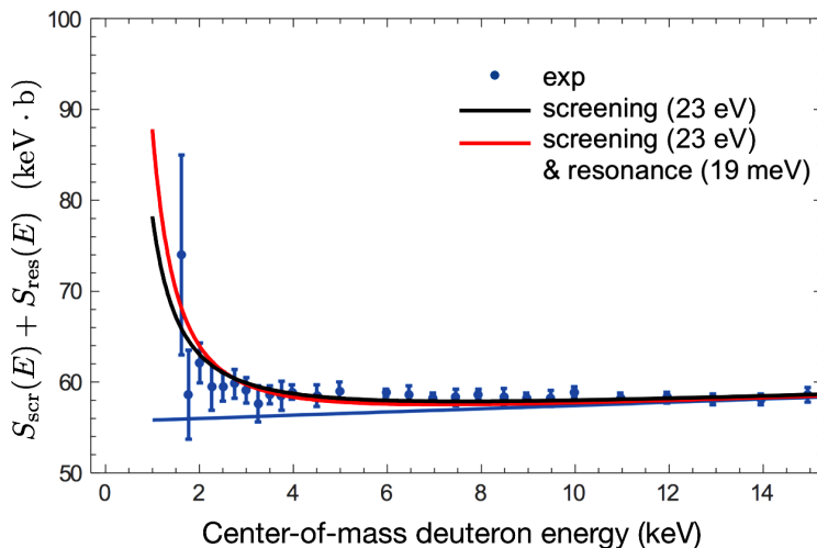
Fig. 2. (Colour on-line) Theoretical S(E) factors connected with screening energy only (black line), as well as together with the resonance contribution (light grey/red line) fitted to gaseous experimental data of Greife et al. [12, 19]. The dark grey/blue line has been proposed by the authors of the experiment as the linear parametrisation of S(E) factor.
