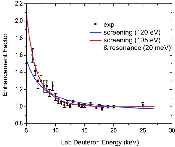
Fig. 1. (Colour on-line) Experimental enhancement factors with theoretical curves fitted to the metallic target experimental data [11].
