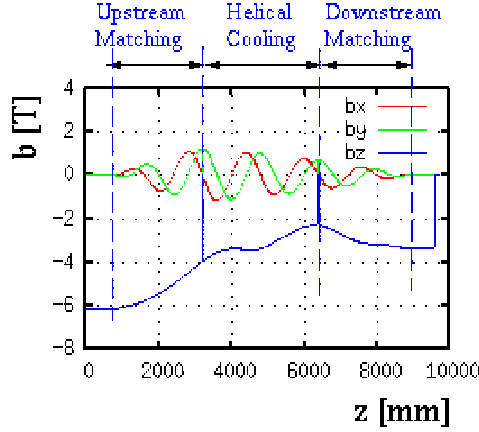
Figure 2: Magnetic field of reference particle in MANX
