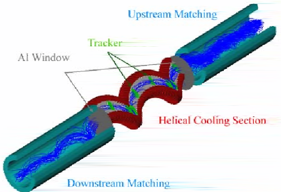
Figure 1: Whole layout of the MANX.
