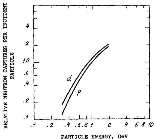
Fig. 2. The calculated relative neutron capture rate in the ^{238}\text{U} component of a large block ( \sim 1 \text{ m}^3 ) of natural uranium bombarded by deuterons (d) and protons (p) normalized to unity for 1 GeV protons.
