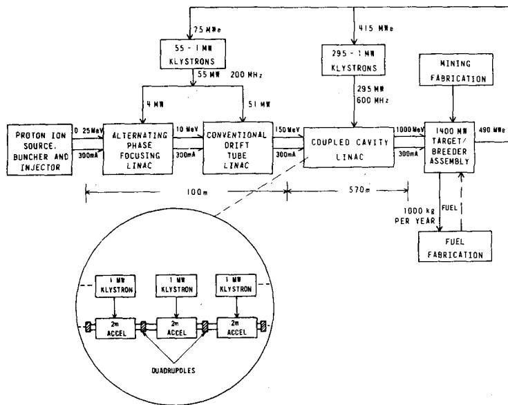
Fig. 3 Schematic of Accelerator Breeder
