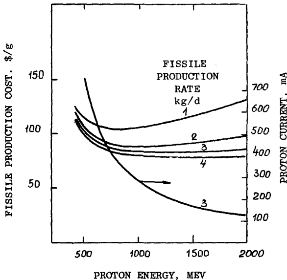
Fig. 4 Calculated unit fissile product costs for production rates 1 to 4 kg per day vs. proton energy. The principal assumptions are: electrical power costs, 10 m$/kWh; target capital, $1000/kWe; interest and depreciation, 10% per year; rf equipment capital $570/kW; accelerator length cost, $50,000/m; maximum peak accelerating field, 1.5 MeV/m, averaged over the accelerator length. Proton beam current as a function of energy to produce 3 kg/d is shown referenced to the right hand ordinate.
