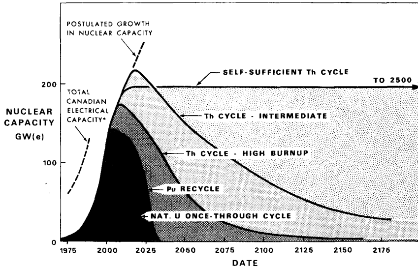
Fig. 1. Nuclear capacity from 3 \times 10^5 tonnes uranium for various CANDU fuel cycles. Characteristics were determined assuming 1 year out-reactor delay for cooling, reprocessing, fabrication and holdup. Fuel burn-up (MWd/kg He) and the total energy produced (GWe-a) for the various cycles are: natural U - 7.5 and 1800, Pu recycling - 18 and 3500, Th - high burn-up (0.88 conversion ratio) - 37.4 and 6900, Th - intermediate (0.96 conversion ratio) - 19.5 and 17000, self-sufficient Th (1.0 conversion ratio) - 10.0 and 79000 (limited by Th supply assumed equal to U supply).
