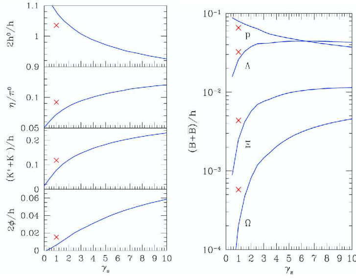
Fig.1. Soft hadron ratios expected at LHC in a non equilibrium scenario. The crosses are the results for the chemical equilibrium [8].
