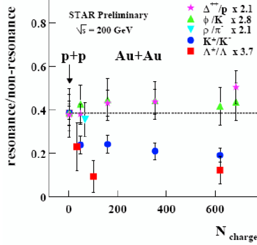
Fig. 3. Resonance over non resonant hadron ratios versus centrality in AuAu and pp collisions at RHIC [15].
