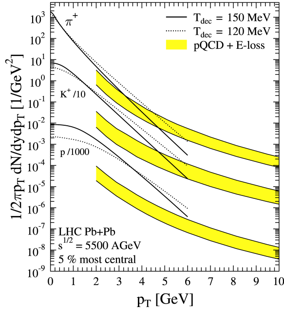
Fig. 2. Comparison between the predictions of the momentum spectra calculated at LHC energies [12]. The hydrodynamical calculations are given for two different decoupling temperatures and the band for the pQCD+Eloss is due to the uncertainties of the extrapolations at the LHC energies.
