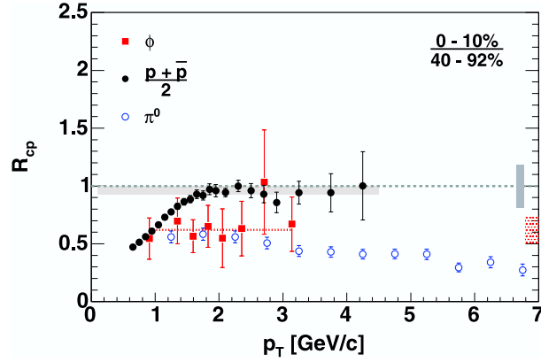
Fig. 4. The nuclear modification factor shows a \phi suppression similar to that of pions [21].
