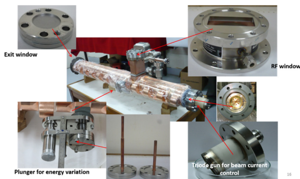
Figure 5: Dual mode linac sub assemblies.
