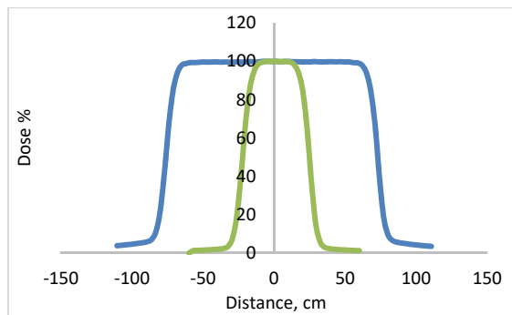
Figure 3: Percentage depth dose curve, (blue) 15x15 cm 2 , (green) 5x5 cm 2 .
