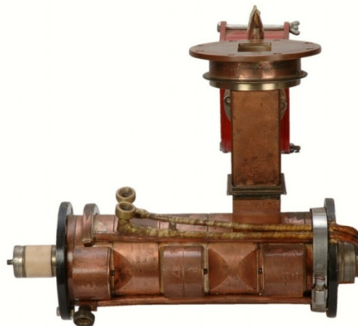
Figure 4: 6 MeV linac.
