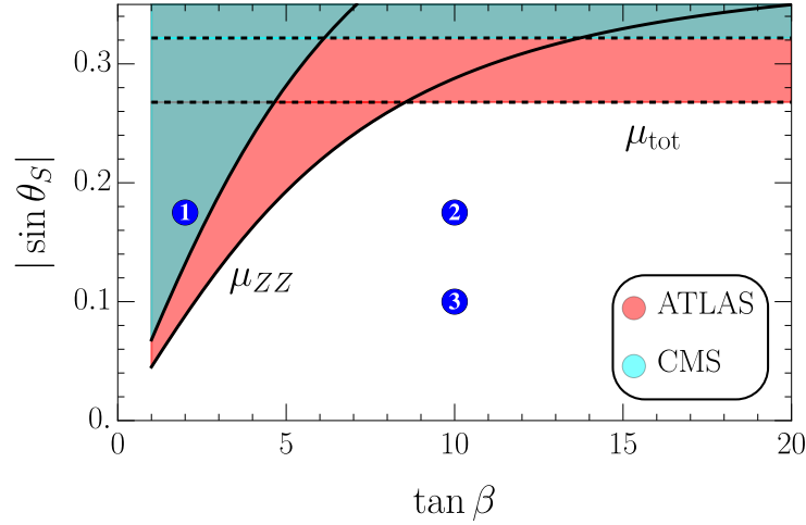
Figure 2. Limit on the sine of the scalar mixing angle \theta_S as a function of \tan \beta . The red (cyan) region is excluded at 95% C.L. by the ATLAS (CMS) measurement of the total and h \rightarrow ZZ^* signal strengths. The blue disks with numbers i correspond to benchmark points BP_i .
