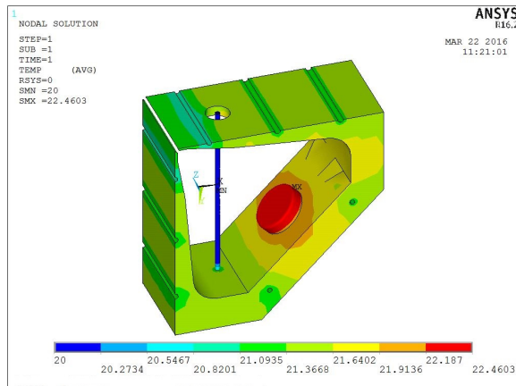
Figure 7: The temperature distributions of the tuners and Pi-mode rods.
