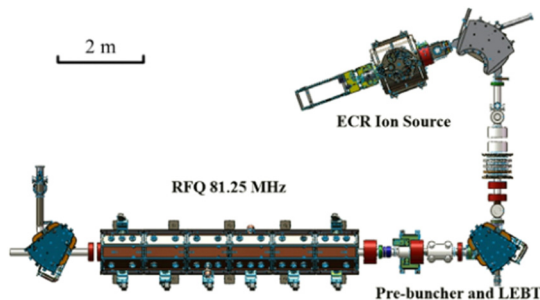
Figure 1: The layout of the LEAF project.
