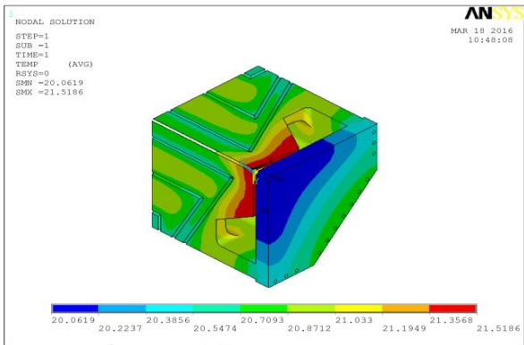
Figure 6: The temperature distributions of the RFQ undercuts.
