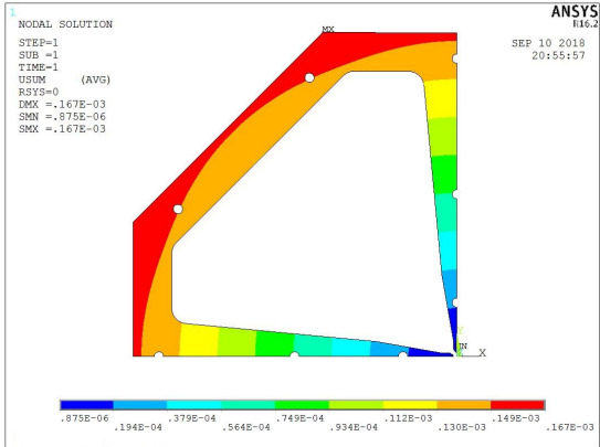
Figure 5: The displacement distribution of the RFQ.
