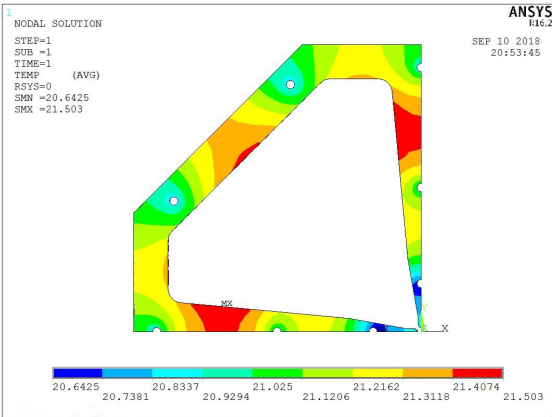
Figure 3: The temperature distribution of the RFQ.
