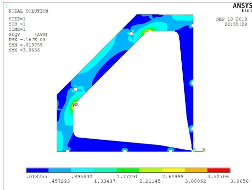
Figure 4: The von-Mises stress distribution of the RFQ.
