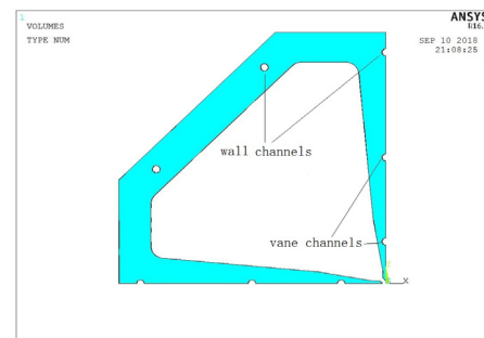
Figure 2: Thin slice model with water cooling channels.
