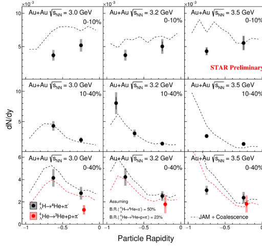
Figure 1. Rapidity distribution of {}^4_{\Lambda}\text{H} and {}^4_{\Lambda}\text{He} in 0-10% and 10-40% Au + Au collision at \sqrt{s_{\text{NN}}} = 3.0 - 3.5 GeV. The symbols represent measurements while the lines represent JAM+Coalescence calculations.
