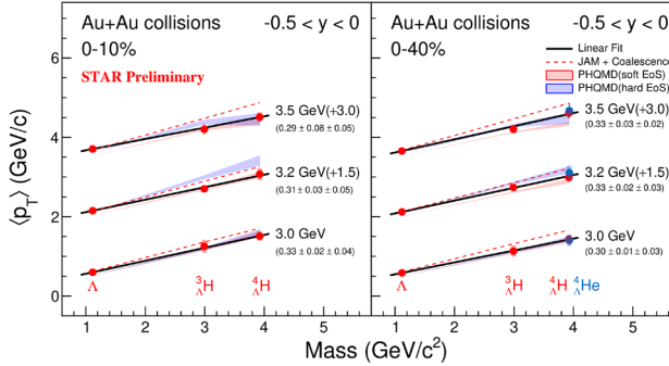
Figure 4. Mass dependence of the mid-rapidity \langle p_T \rangle for \Lambda , {}^3_\Lambda\text{H} , {}^4_\Lambda\text{H} and {}^4_\Lambda\text{He} , from the \sqrt{s_{NN}} = 3.0 - 3.5 GeV in 0-10% and 0-40% Au+Au collisions. The symbols represent measurements while the lines represent JAM+Coalescence and PHQMD model calculations. The numbers in parentheses next to the energy represent the vertical shifts, while the numbers in the lower parentheses indicate the slopes of the linear fits.
