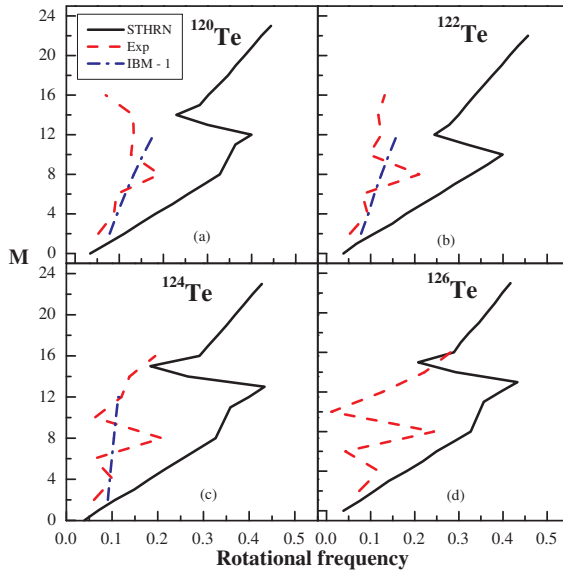
Fig. 5. (Color online) Angular momentum M as a function of rotational frequency \omega \hbar / \text{MeV} for (a) ^{120}\text{Te} (b) ^{122}\text{Te} , (c) ^{124}\text{Te} and, (d) ^{126}\text{Te} at T = 3.0 MeV. The solid black line represent the moment of inertia value calculated from the STHRn method, the dashed red line corresponds to experimental data [2, 10] and the dash-dotted blue line represents the IBM-1 data [7].
