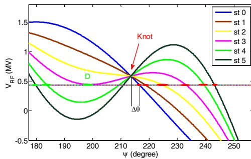
Figure 2: Twin RF bucket creation with synchrotron phase deviation. (From st 0 to st 5, the normalized RF voltages [\widehat{V}_m, \widehat{V}_h] / \widehat{V}_m(0) is [1, 0.1], [1, 0.2], [1, 0.4], [1, 0.58], [1, 0.8] and [1, 1] respectively).
