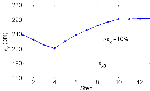
Figure 5: Equilibrium horizontal emittance during the injection process.
