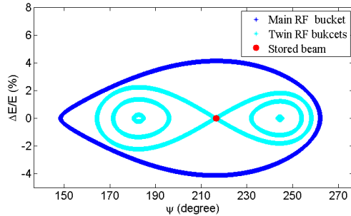
Figure 1: Twin RF buckets creation by two RF systems.
