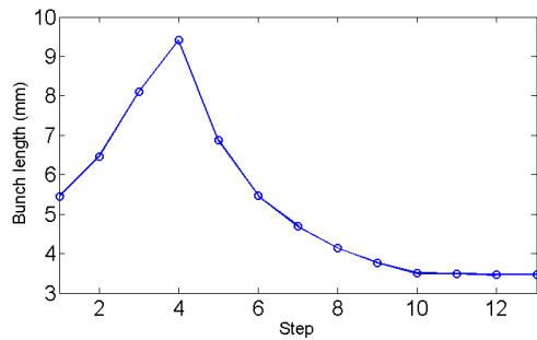
Figure 4: Bunch length evolution of stored bunch.
