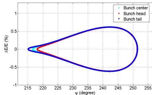
Figure 3: Tracking of longitudinal motion of injected bunch at the dumping point \Delta\theta=7 degree.
