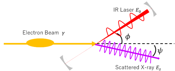
Figure 1: Schematic of LCS.
