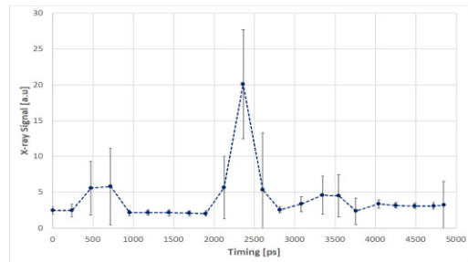
Figure 10: X-ray signal as a function of timing.
