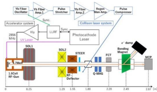
Figure 9: Experiment setup in LCS.
