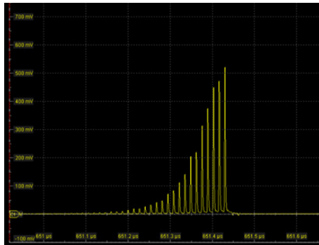
Figure 8: Pulse build-up regenerative amplifier.
