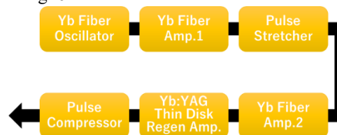
Figure 6: Schematic of collision laser system.
