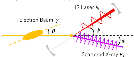
Figure 3: Schematic of crab crossing LCS.
