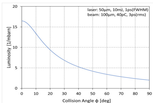
Figure 2: Luminosity dependence on collision angle.
