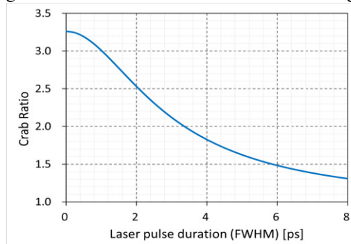
Figure 5: Laser pulse duration and crab ratio.
