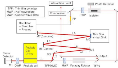
Figure 7: Schematic of thin-disk regenerative amplifier.
